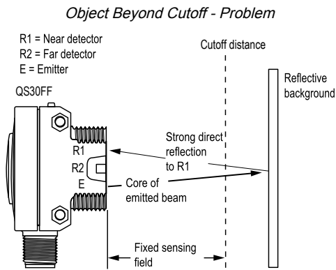
A reflective background object in this position or moving across the sensor face in this axis and direction may cause a false sensor response.
