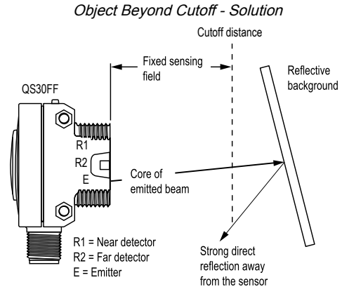
A reflective background object in this position or moving across the sensor face in this axis is ignored.
