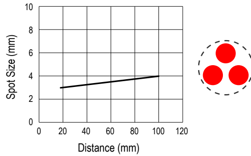
Q2XLAF100 (Laser) Typical Emitter Spot Diameter vs. Distance
