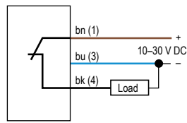
PNP Models, Dark Operate
