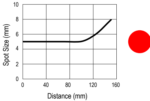
Q2XAF150 (LED) Typical Emitter Spot Diameter vs. Distance
