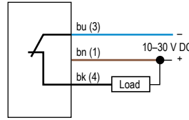
NPN Models, Dark Operate
