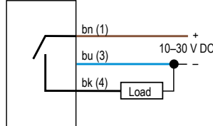
PNP Models, Dark Operate
