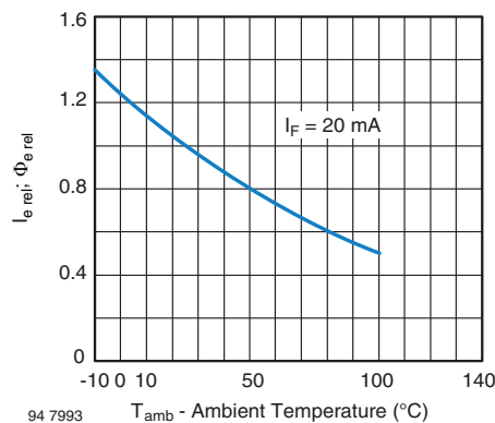
Fig. 6 - Relative Radiant Intensity/Power vs. Ambient Temperature
