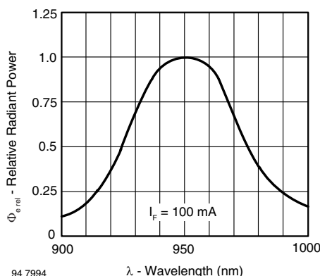
Fig. 7 - Relative Radiant Power vs. Wavelength
