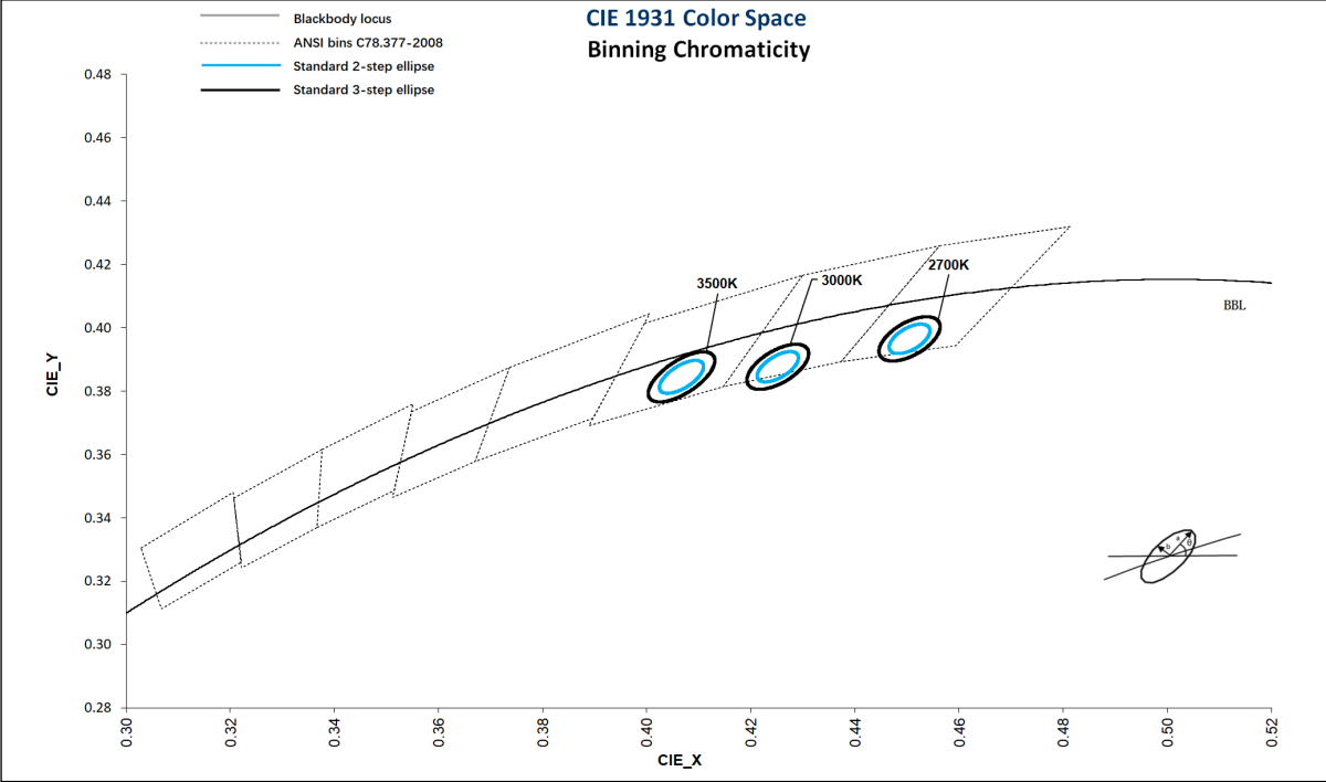
Chromaticity Binning Diagram 1 - TC/TA62 Sensus (BBBL)
