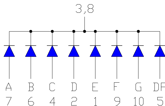
OPS-S5111 (Common Cathode)
