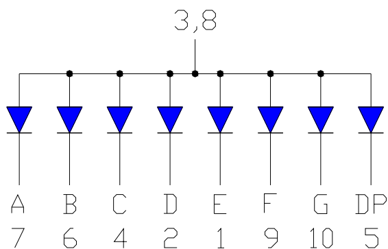
OPS-S5110 (Common Anode)
