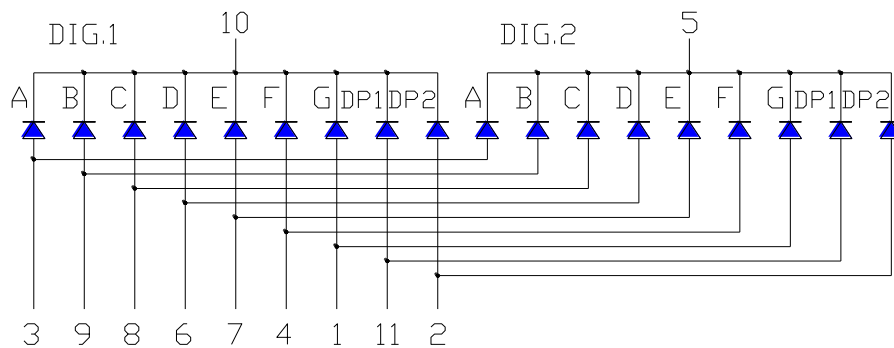
OPS-D2813 (Common Cathode)
