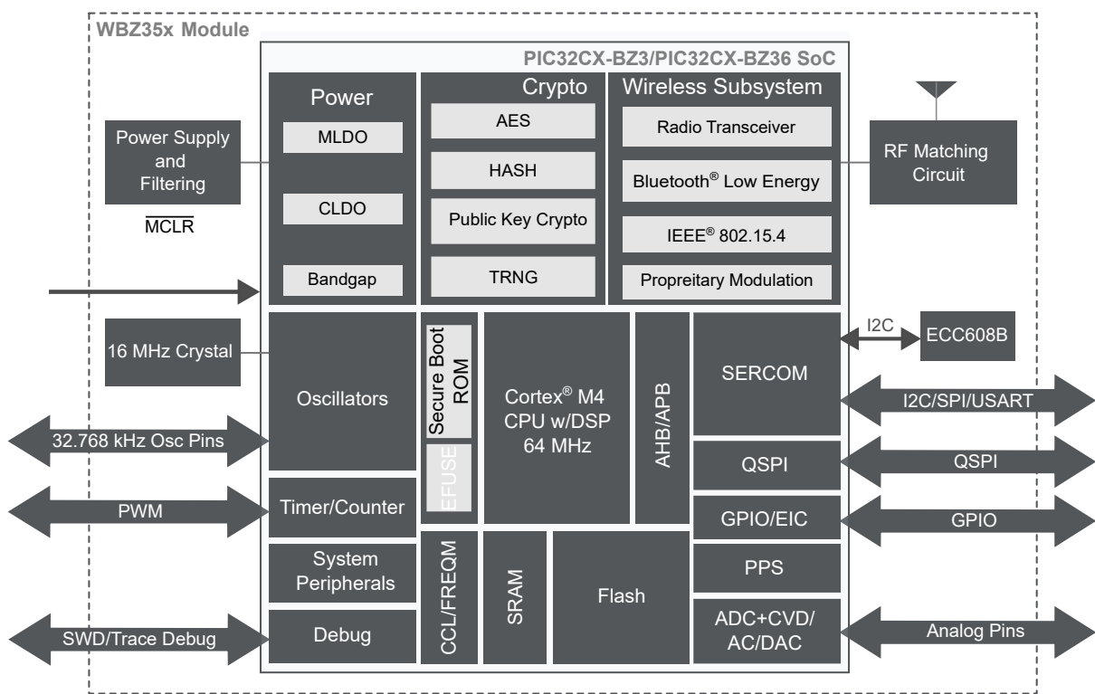
Figure 4-1. WBZ35x Module Block Diagram
