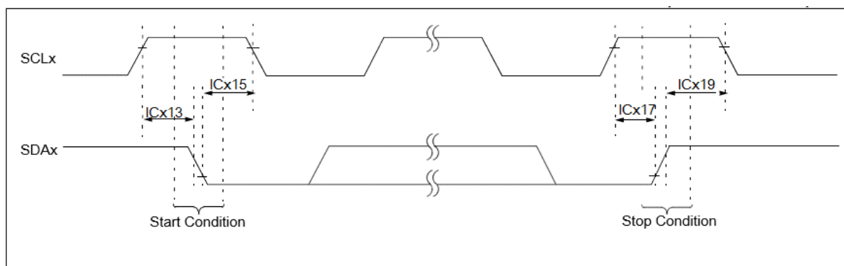
Figure 43-50. I 2 C Start/Stop Bits Client Mode AC Timing Diagram
