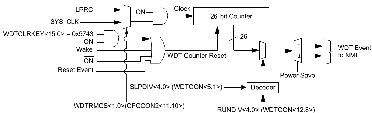
Figure 19-1. Block Diagram
