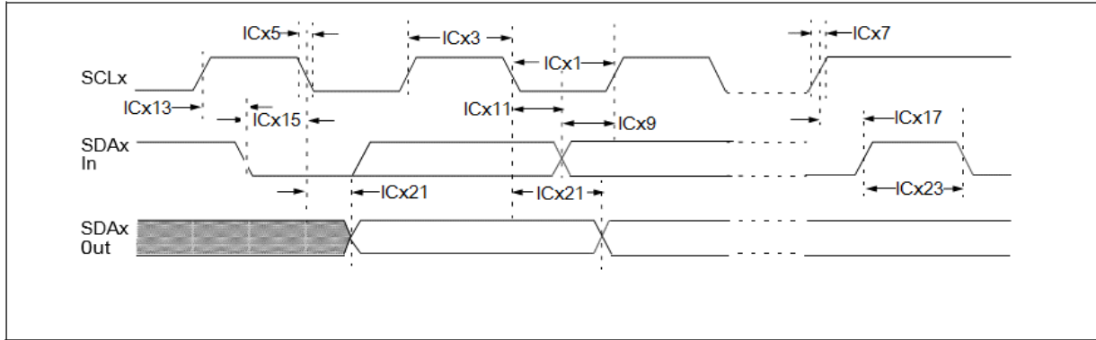
Figure 43-51. I 2 C Bus Data Client Mode AC Timing Diagram
