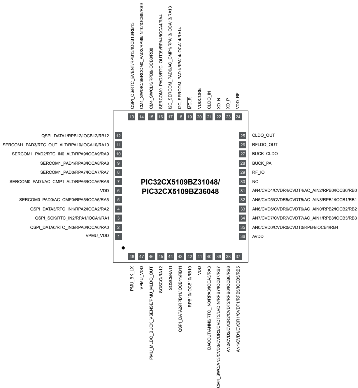
Figure 3-2. PIC32CX5109BZ31048/PIC32CX5109BZ36048 SoC Pinout Diagram
