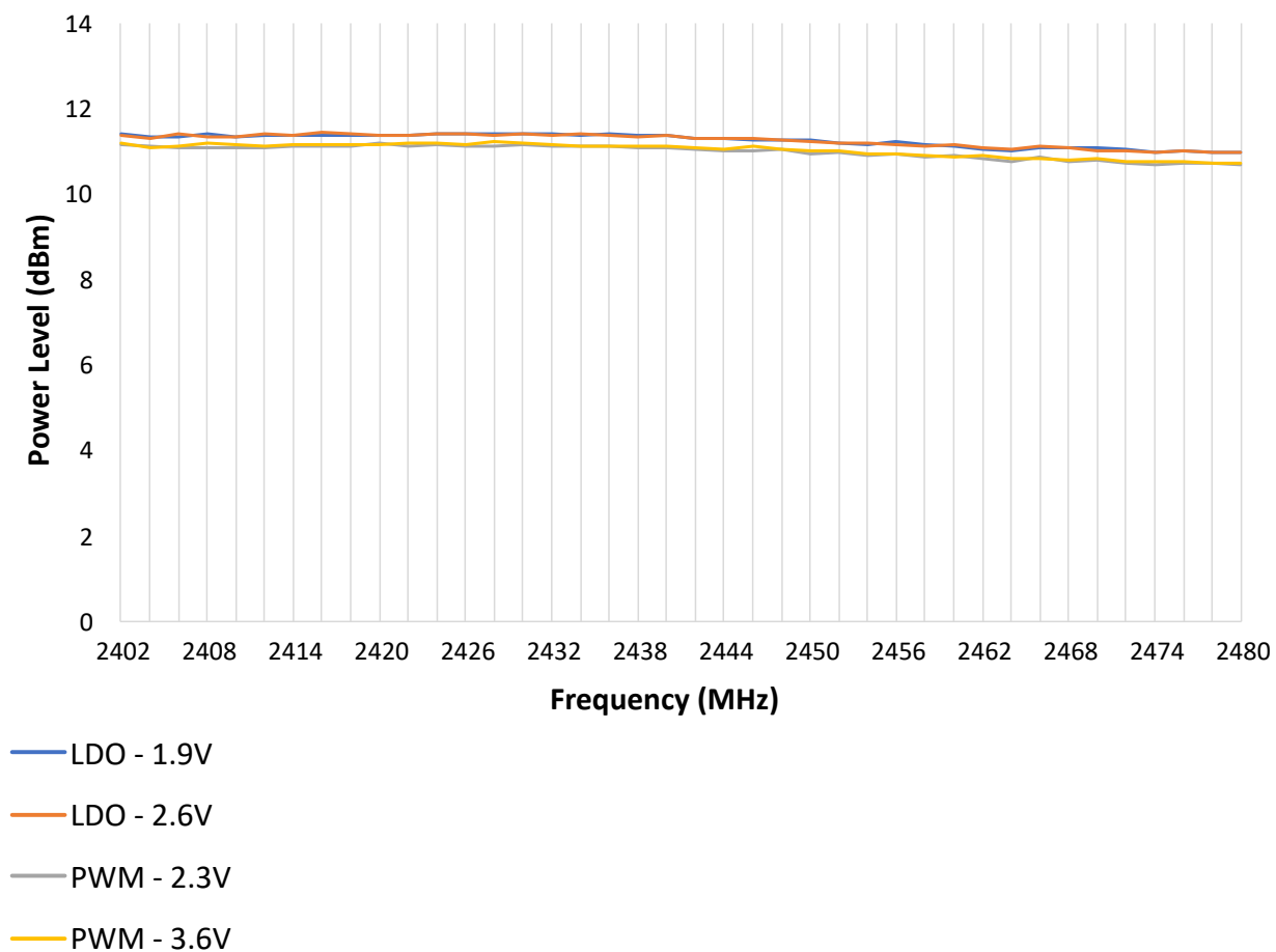
Figure 43-62. Bluetooth Low Energy 1M Transmit Power vs. Frequency
