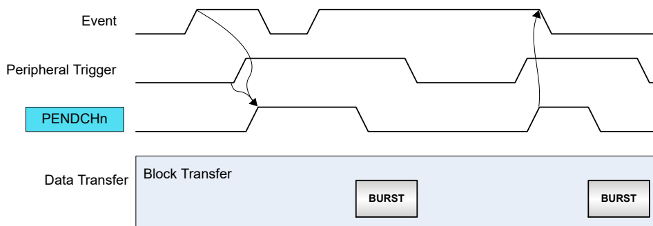
Figure 26-14. Conditional Event with Burst Peripheral Triggers
