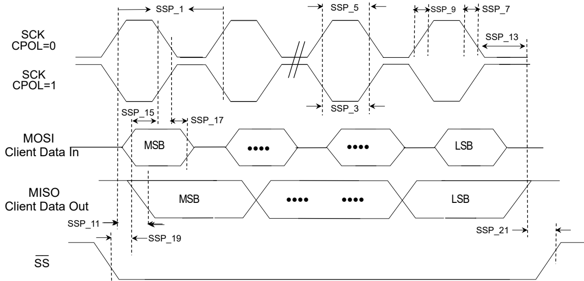
Figure 43-6. SPI Client Module CPHA = 1 Timing Diagrams
