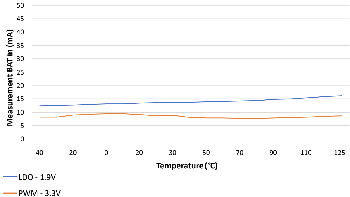
Figure 43-70. WBZ35x Module Bluetooth Low Energy Receive Current vs. Temperature
