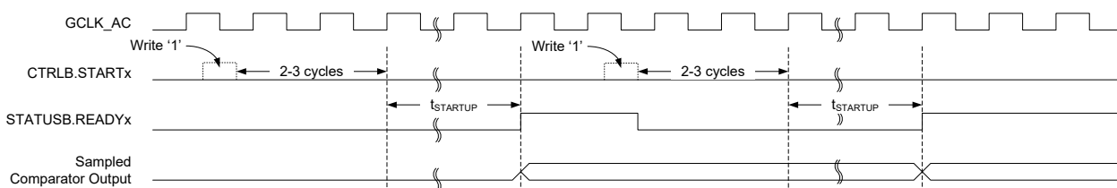
Figure 38-3. Single-Shot Example
