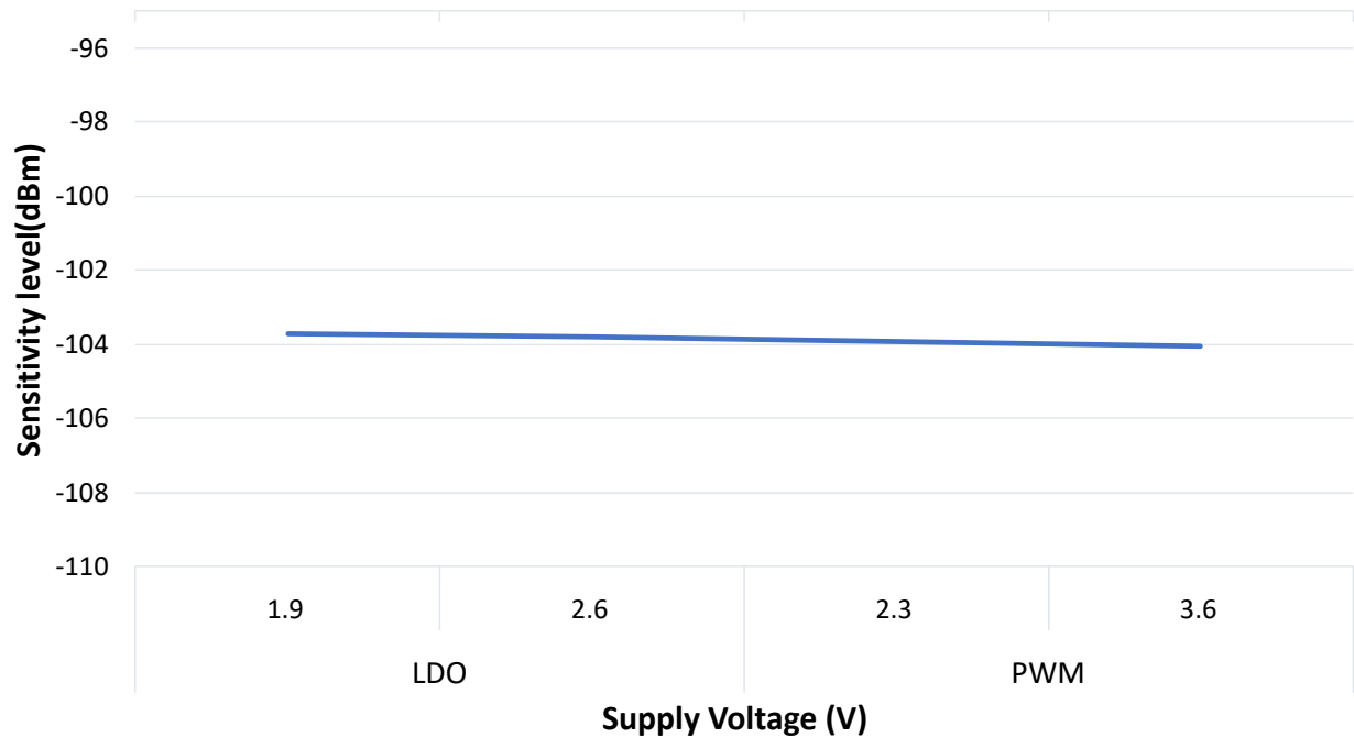
Figure 43-79. Zigbee Receive Sensitivity vs. Voltage
