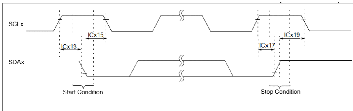
Figure 43-48. I 2 C Start/Stop Bits Host Mode AC Timing Diagram
