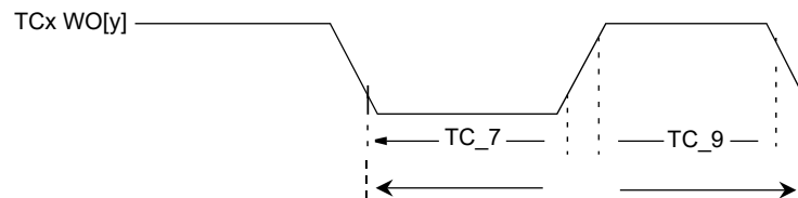
Figure 43-53. TCx Timer Capture Output Module AC Timing Diagram
