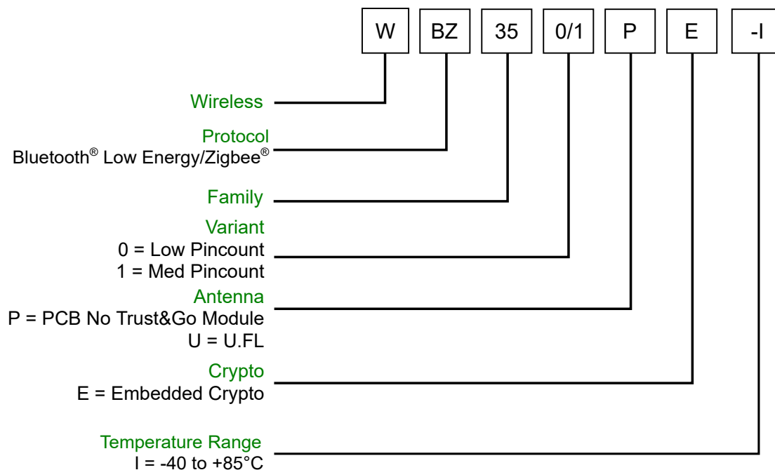
Figure 1-3. WBZ35x Module Ordering Information
