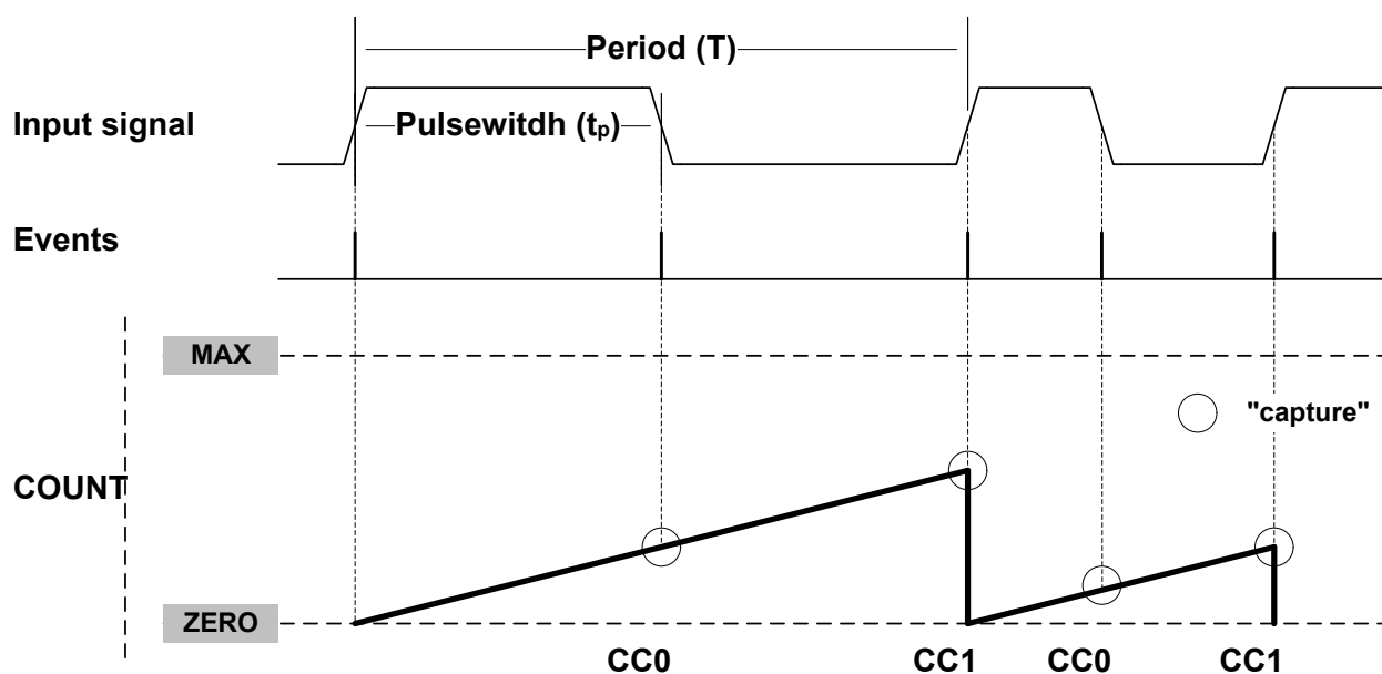
Figure 40-13. PWP Capture
