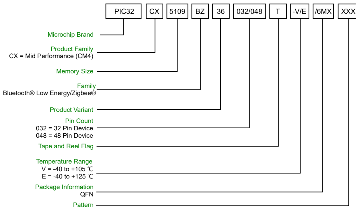
Figure 1-2. PIC32CX-BZ36 Ordering Information
