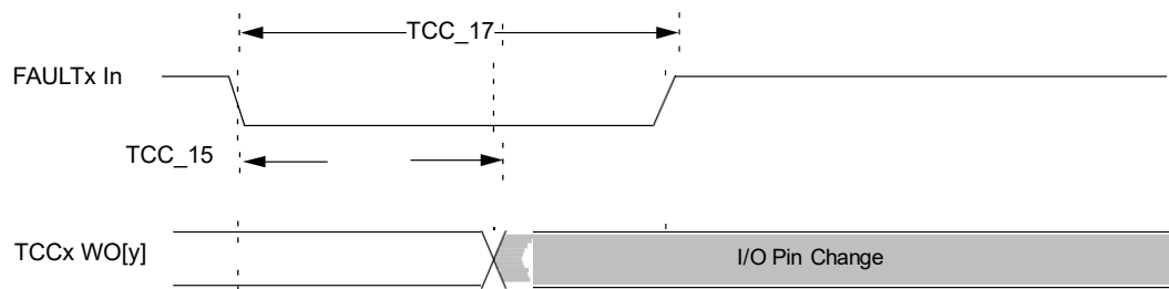
Figure 43-56. TCC_x Timer Compare Fault Output Module AC Timing Diagram
