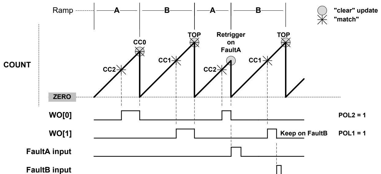
Figure 41-20. RAMP2 Critical Operation With More Than 2 Channels
