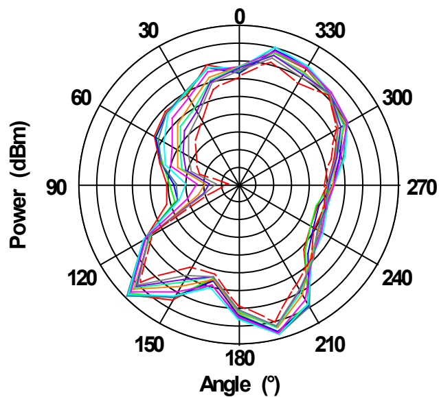
Figure 4-15. WBZ351 Antenna Radiation Pattern when \Theta = 90^\circ
