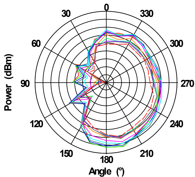
Figure 4-11. WBZ350 Antenna Radiation Pattern when \Theta = 90^\circ
