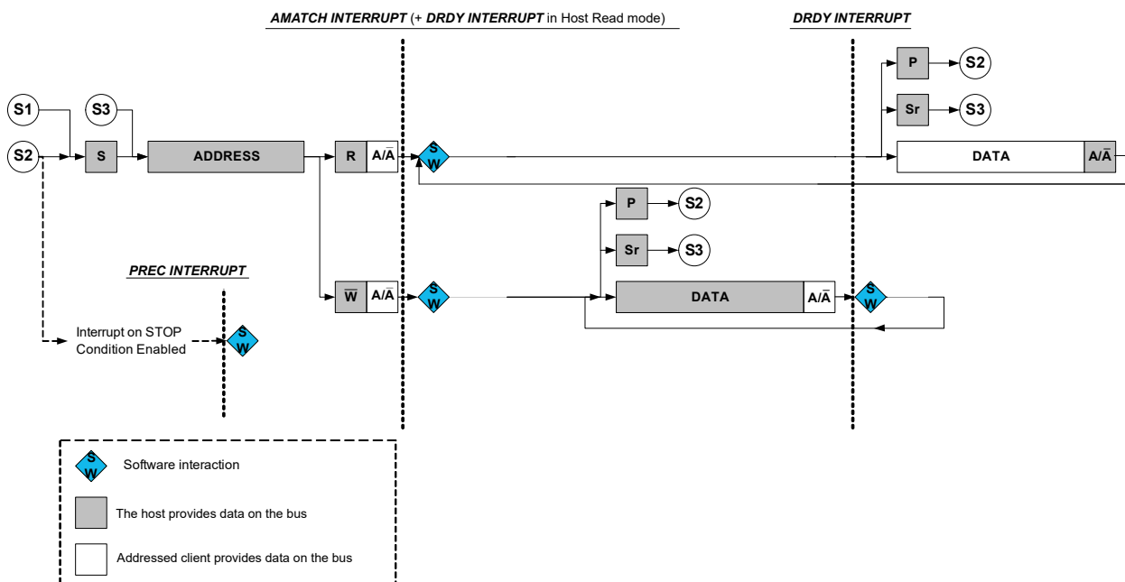
Figure 34-9. I 2 C Client Behavioral Diagram (SCLSM = 1)
