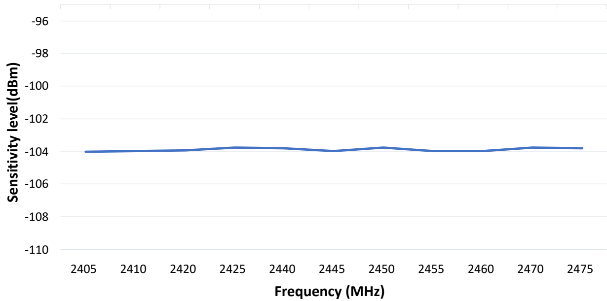
Figure 43-77. WBZ35x Module Zigbee Receive Sensitivity vs. Frequency
