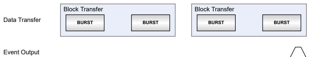
Figure 26-16. Block Event Output Generation
