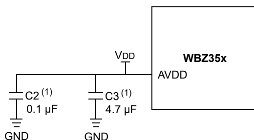
Figure 4-5. Recommended Module Power Supply Connections
