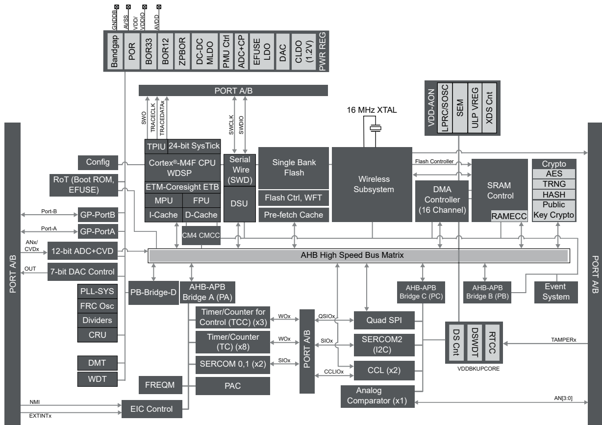
Figure 3-1. PIC32CX-BZ3/PIC32CX-BZ36 SoC Block Diagram
