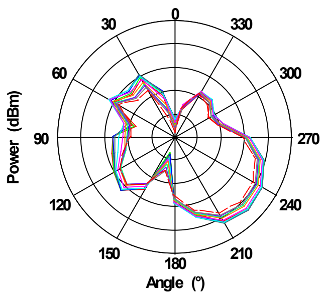
Figure 4-9. WBZ350 Antenna Radiation Pattern when \Phi = 0^\circ
