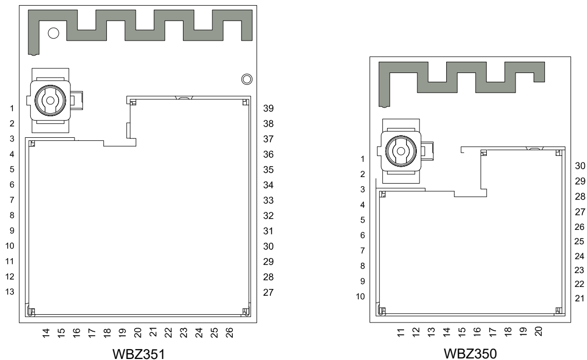
Figure 4-2. WBZ351 and WBZ350 Module Ping Diagram (Top View)
