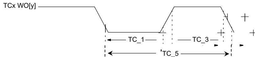
Figure 43-52. TCx Timer Capture Input Module AC Timing Diagram
