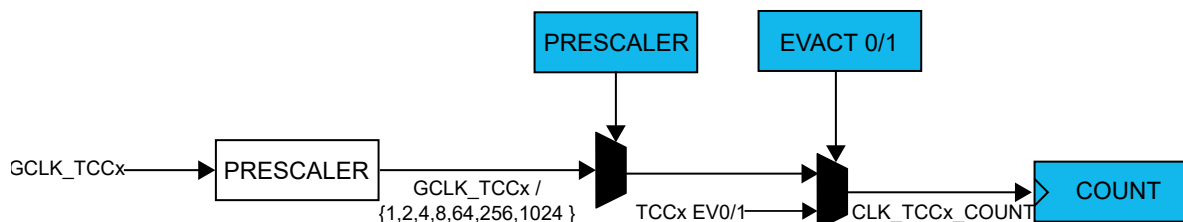
Figure 41-2. Prescaler
