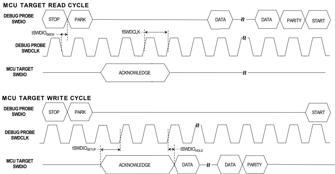
Figure 43-57. SWD 2-Wire Read/Write AC Timing Diagram
