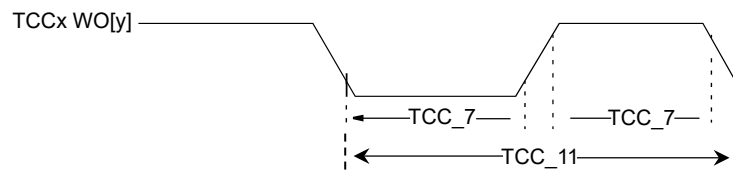
Figure 43-55. TCCx Timer Capture Output Module AC Timing Diagram
