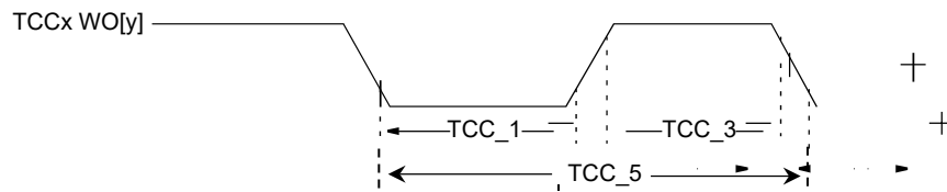
Figure 43-55. TCCx Timer Capture Output Module AC Timing Diagram
