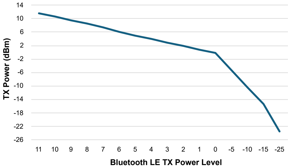
Figure 43-59. Bluetooth Low Energy Transmit Power vs. Transmit Power Level
