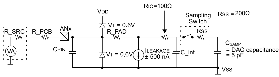
Figure 36-12. 12-bit ADC Analog Input Model
