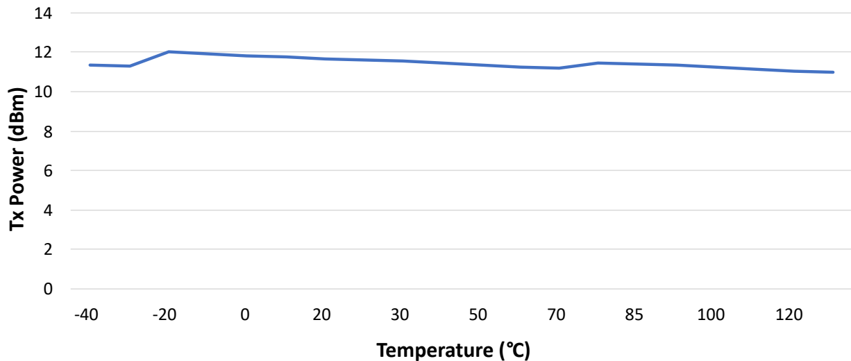
Figure 43-71. Zigbee Transmit Power vs. Temperature
