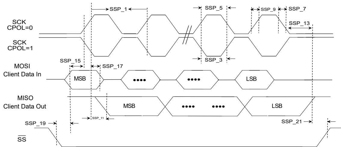
Figure 43-5. SPI Client Module CPHA = 0 Timing Diagrams
