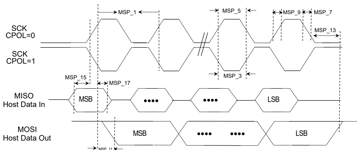
Figure 43-3. SPI Host Module CPHA = 0 Timing Diagrams
