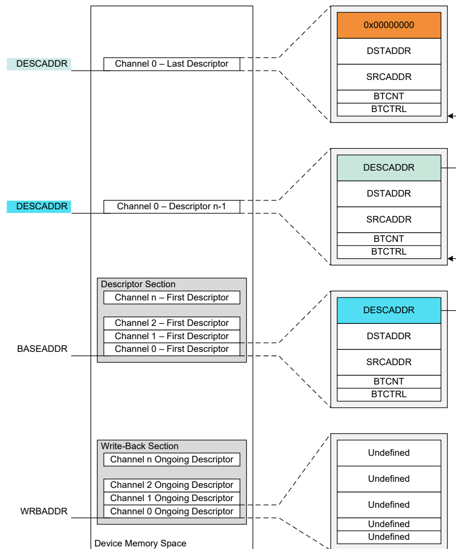
Figure 26-3. Memory Sections
