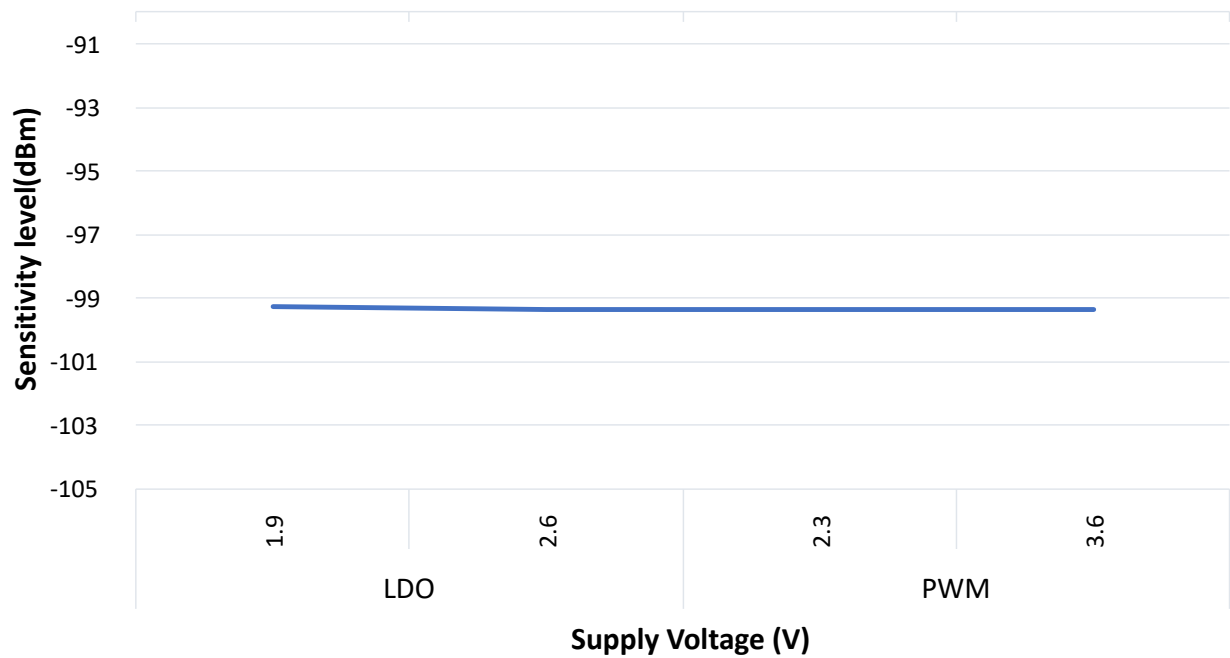
Figure 43-66. Bluetooth Low Energy Receive Sensitivity vs. Voltage
