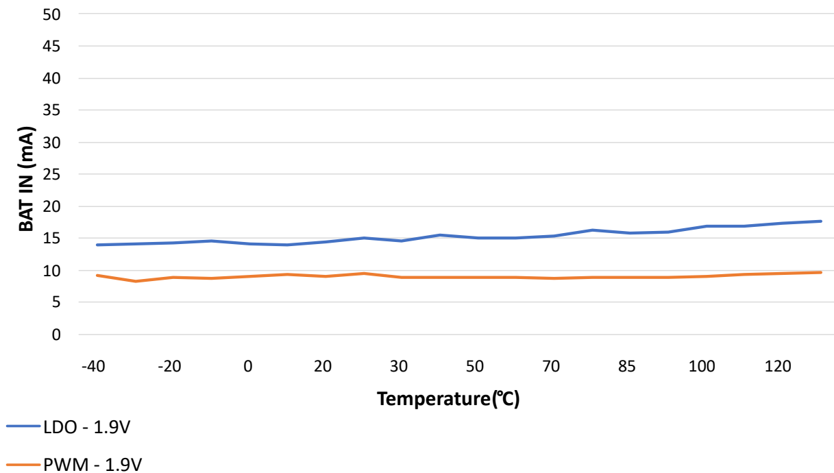
Figure 43-83. Zigbee Receive Current vs. Temperature
