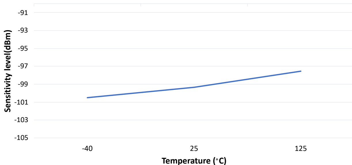
Figure 43-61. WBZ35x Module Bluetooth Low Energy Receive Sensitivity vs. Temperature
