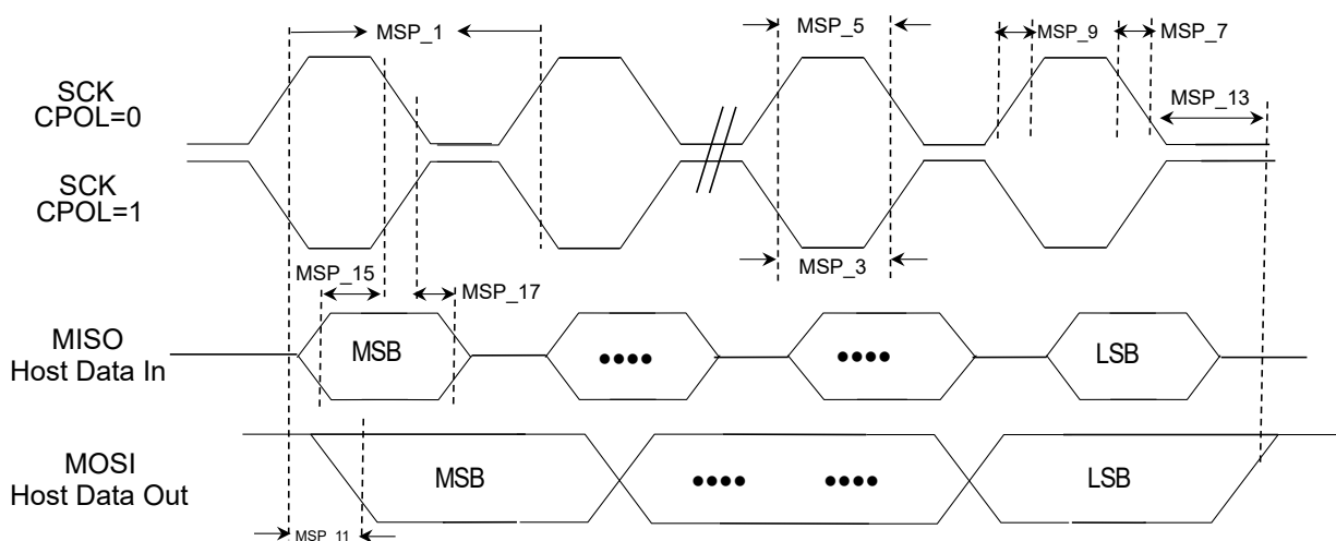
Figure 43-45. SPI Host Module CPHA = 1 Timing Diagrams
