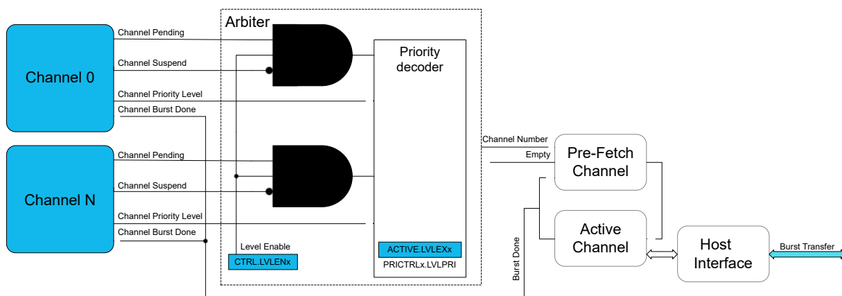
Figure 26-4. Arbiter Overview
