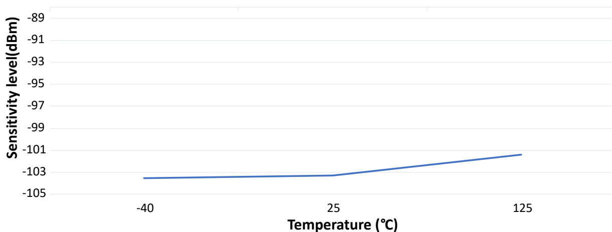
Figure 43-33. WBZ35x Module Zigbee Receive Sensitivity vs. Temperature
