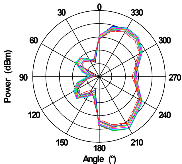
Figure 4-11. WBZ350 Antenna Radiation Pattern when \Theta = 90^\circ
