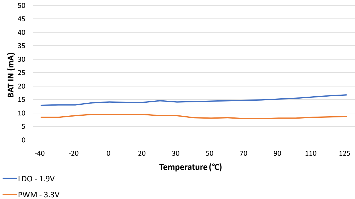
Figure 43-84. WBZ35x Module Zigbee Receive Current vs. Temperature
