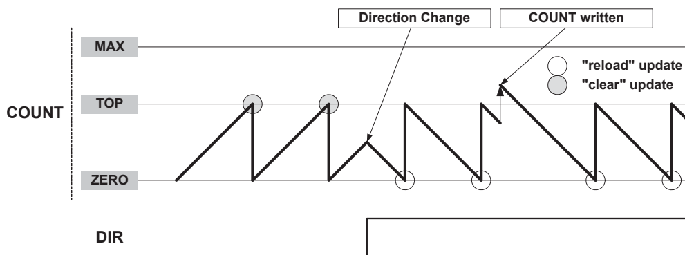
Figure 41-3. Counter Operation
