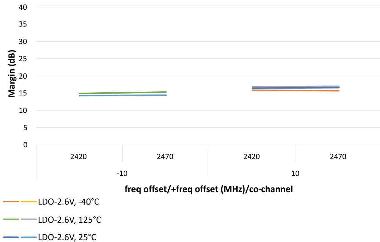
Figure 43-81. Zigbee ACR +-10M Margin
