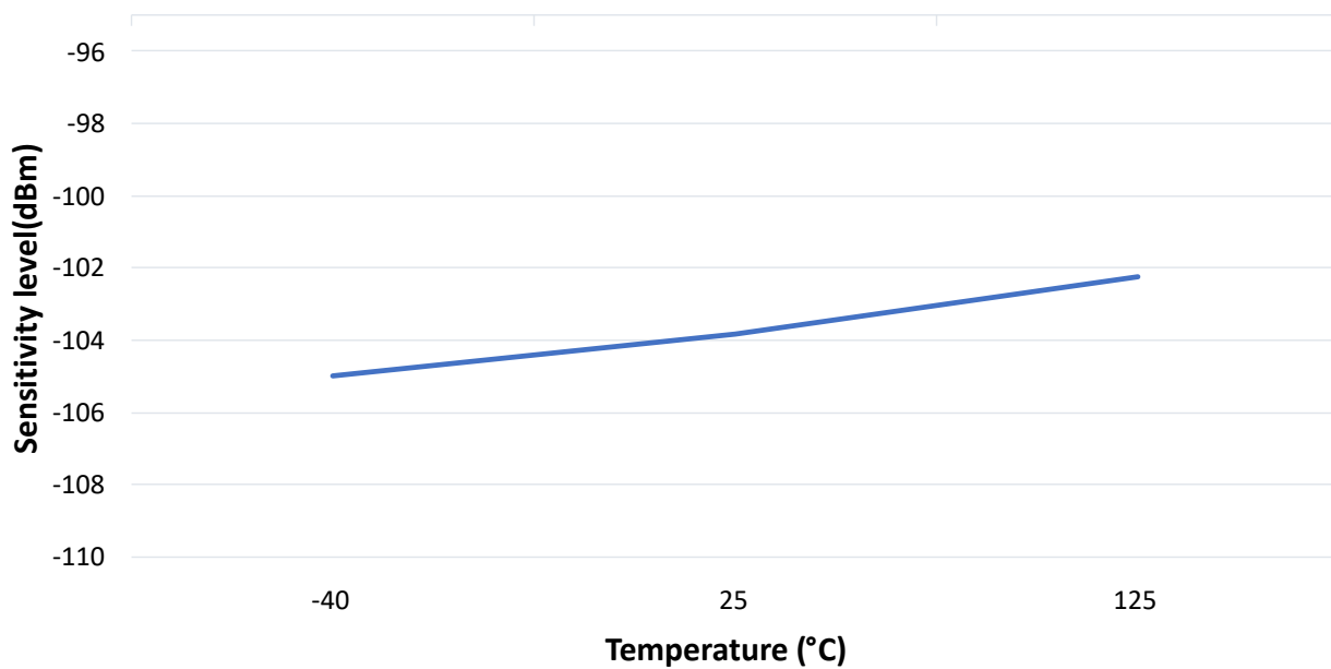
Figure 43-73. Zigbee Receive Sensitivity vs. Temperature
