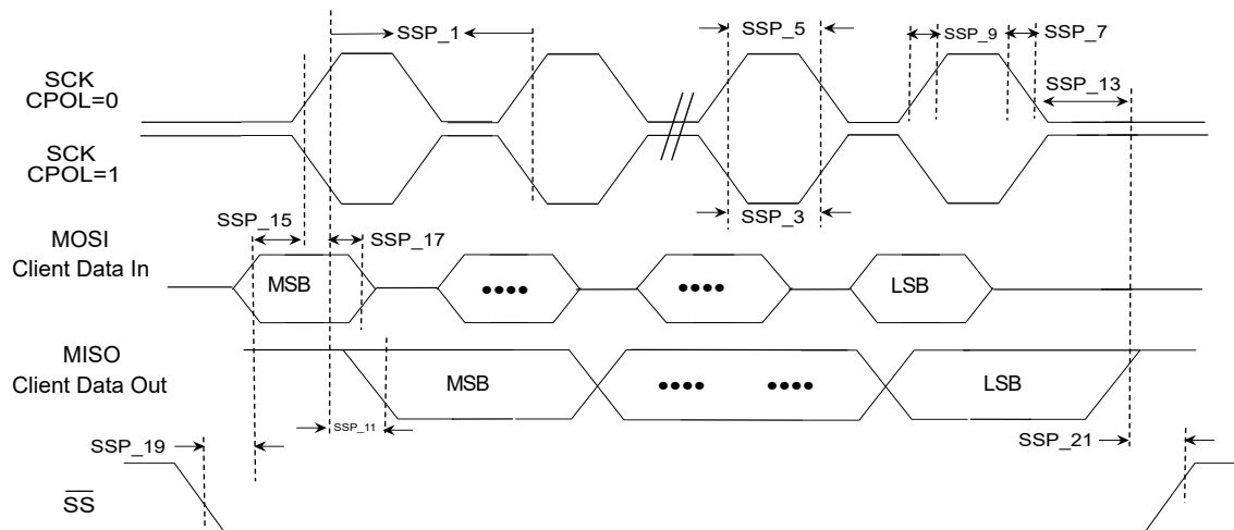
Figure 43-46. SPI Client Module CPHA = 0 Timing Diagrams
