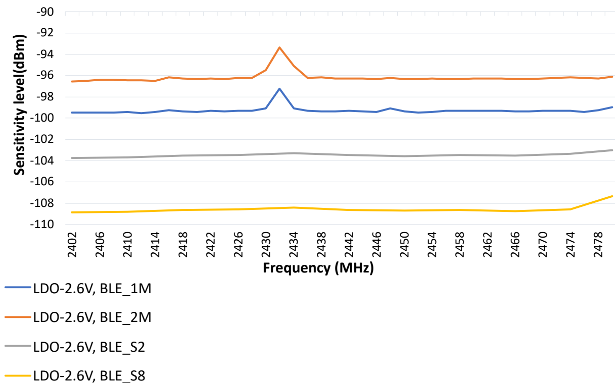
Figure 43-64. WBZ35x Module Bluetooth Low Energy Receive Sensitivity vs. Frequency
