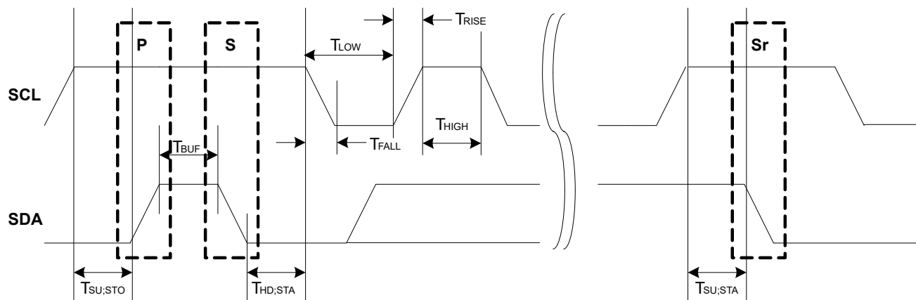
Figure 34-7. SCL Timing
