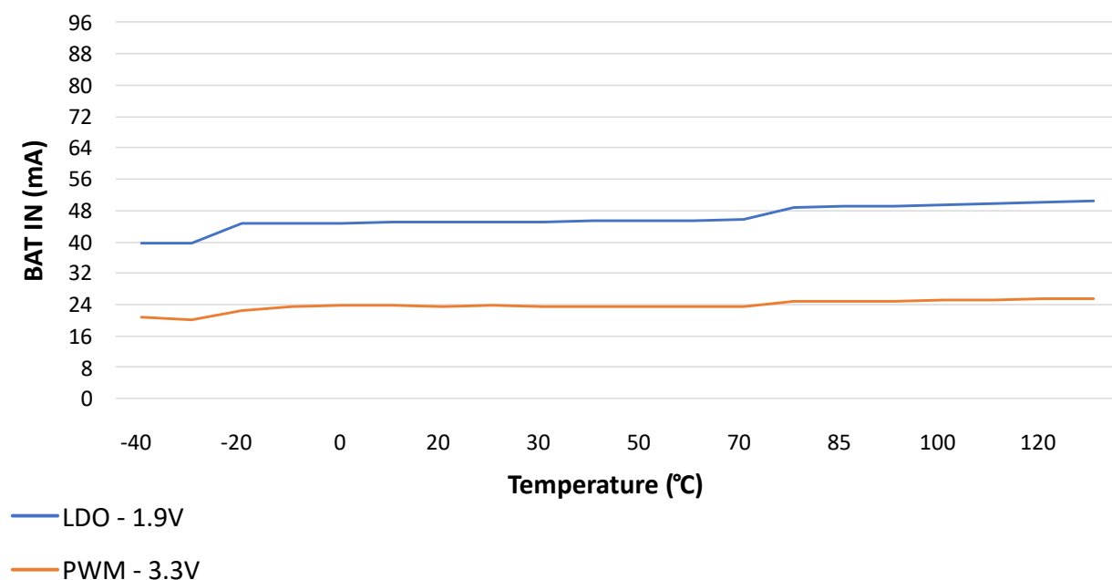
Figure 43-68. Bluetooth Low Energy Transmit Current vs. Temperature
