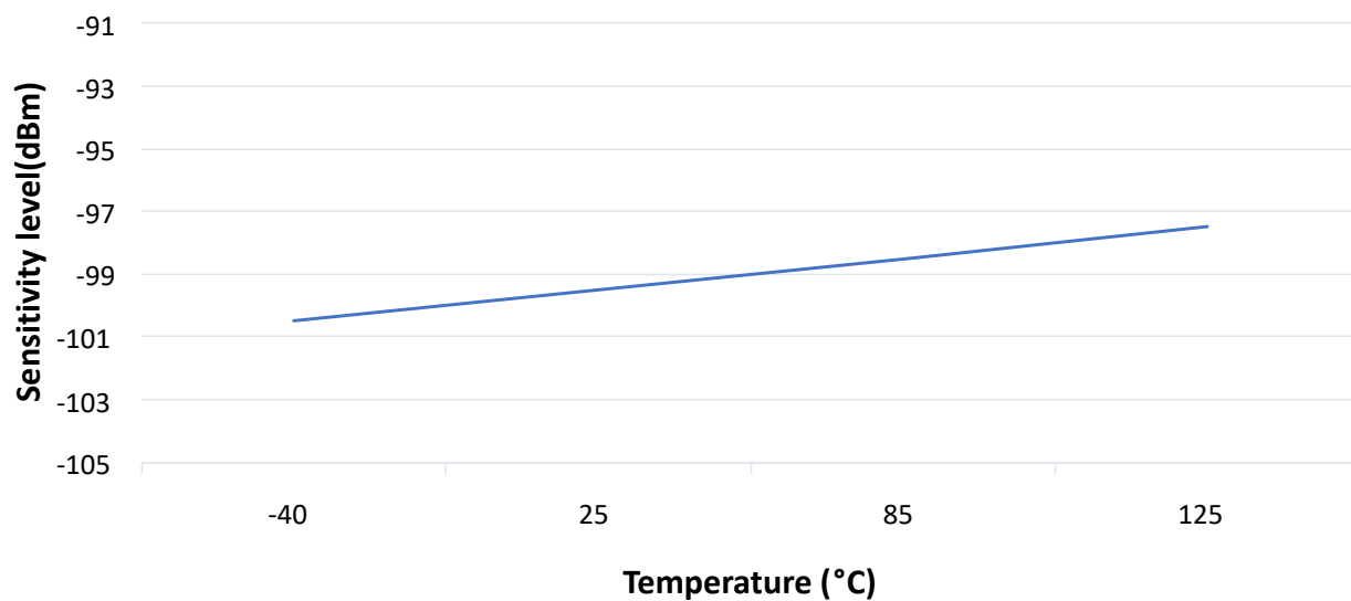
Figure 43-61. WBZ35x Module Bluetooth Low Energy Receive Sensitivity vs. Temperature
