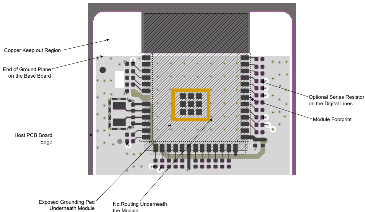
Figure 4-8. Example of Host Board on Top Layer
