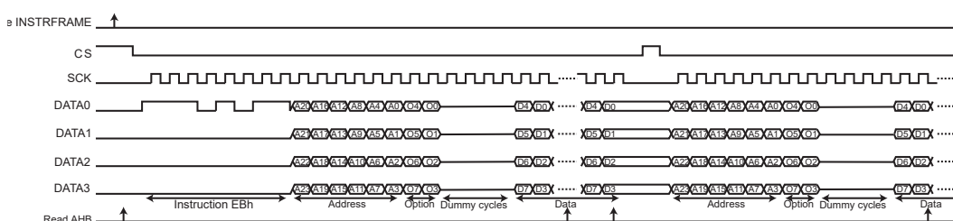
Figure 35-18. Instruction Transmission Waveform 7
