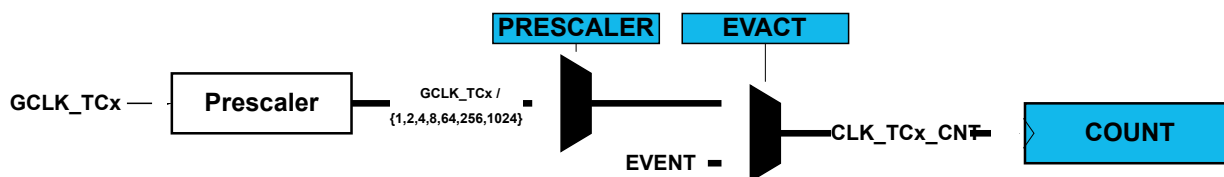
Figure 40-2. Prescaler
