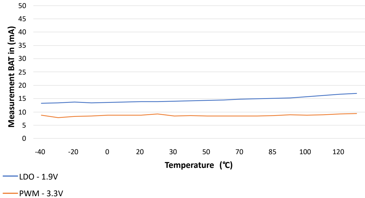
Figure 43-70. WBZ35x Module Bluetooth Low Energy Receive Current vs. Temperature
