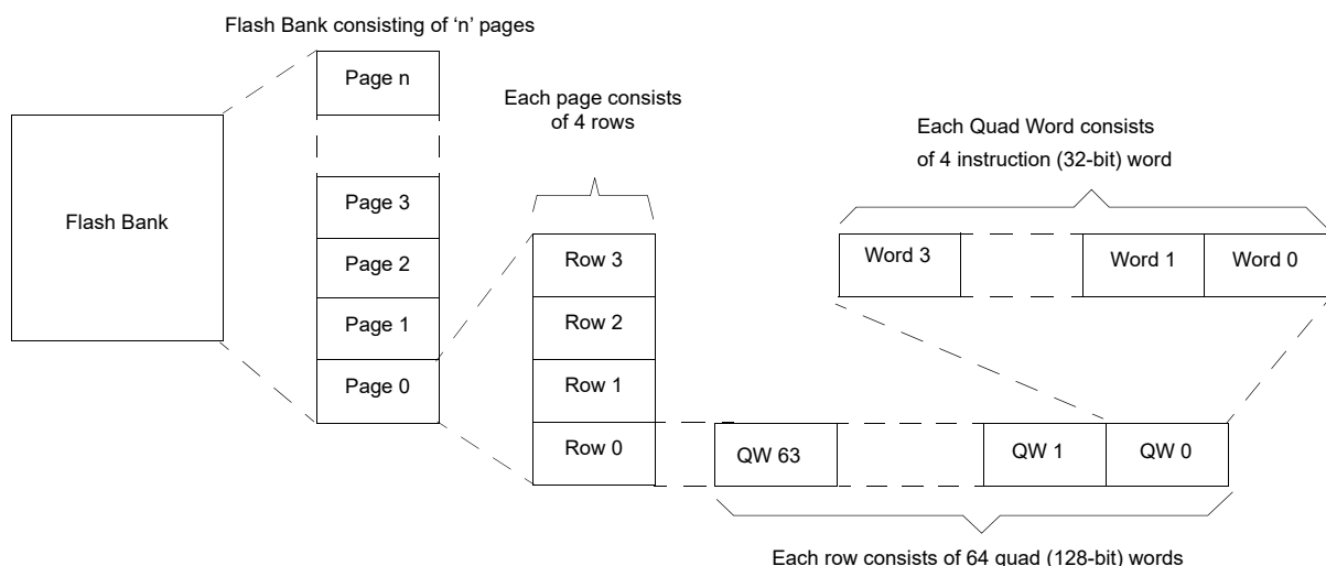
Figure 15-2. Flash Construction
