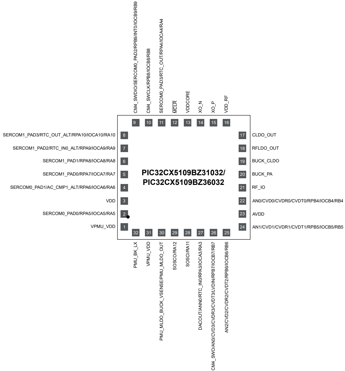
Figure 3-3. PIC32CX5109BZ31032/PIC32CX5109BZ36032 SoC Pinout Diagram
