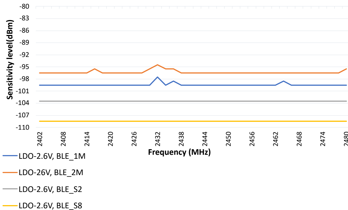
Figure 43-64. WBZ35x Module Bluetooth Low Energy Receive Sensitivity vs. Frequency
