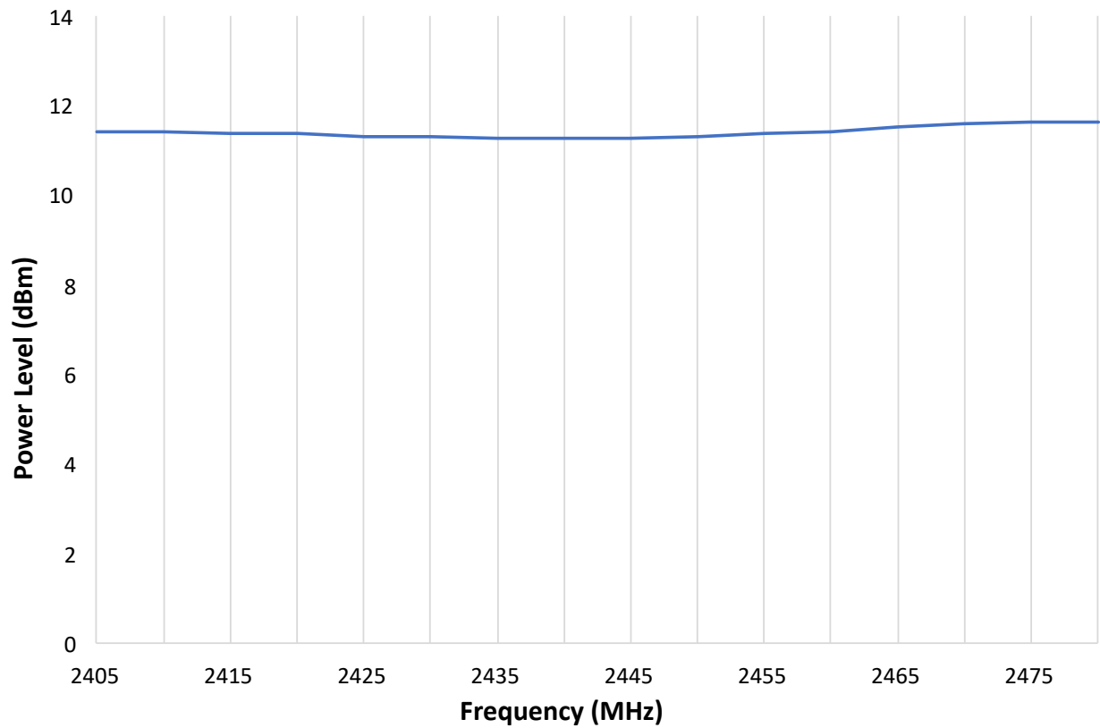
Figure 43-75. Zigbee-1M Transmit Power vs. Frequency
