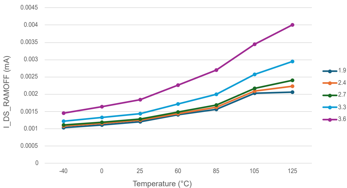
Figure 49-13. Deep Sleep Current RAM OFF
