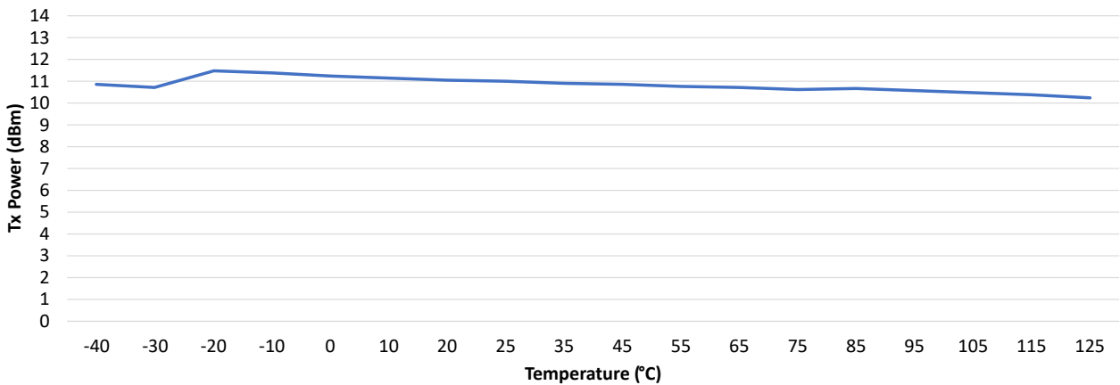
Figure 49-35. Bluetooth Low Energy Transmit Power vs. Temperature
