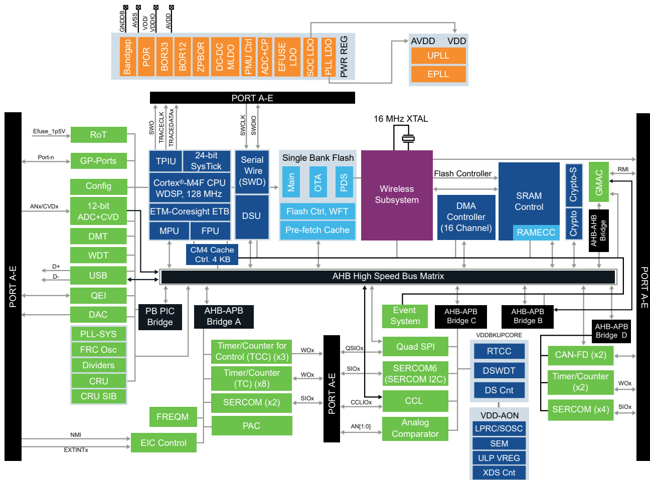
Figure 4-1. PIC32CX-BZ6 SoC Block Diagram
