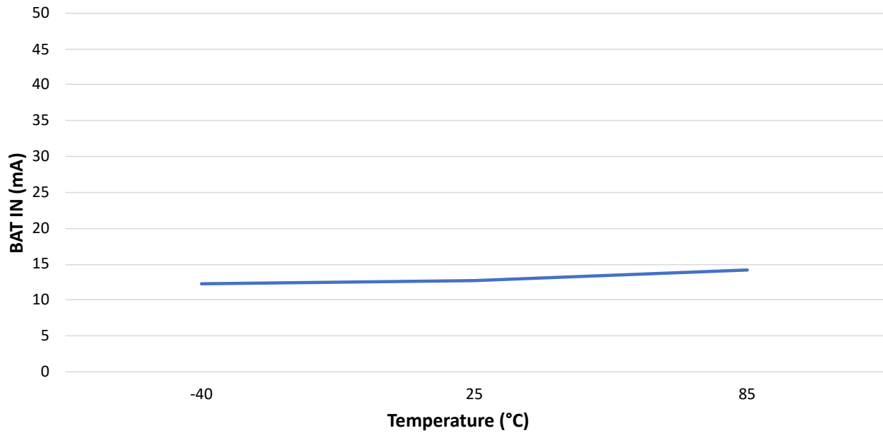
Figure 49-58. Module Zigbee Receive Current vs. Temperature
