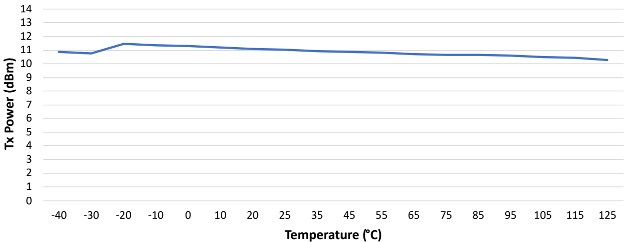
Figure 49-47. Zigbee Transmit Power vs. Temperature
