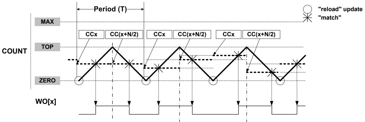
Figure 42-8. Dual-Slope Critical Pulse Width Modulation (N=CC_NUM)
