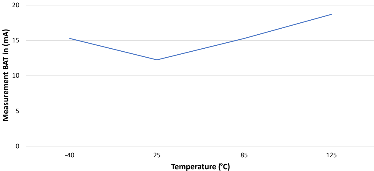
Figure 49-42. Bluetooth Low Energy Receive Current vs. Temperature
