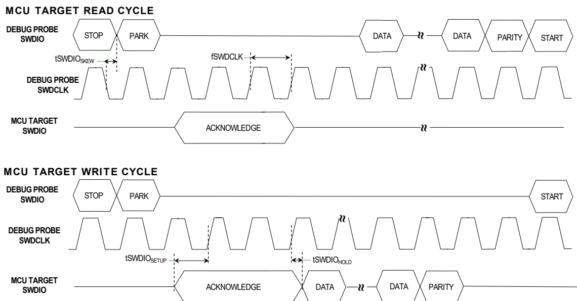
Figure 49-34. SWD Two-Wire Read/Write AC Timing Diagram
