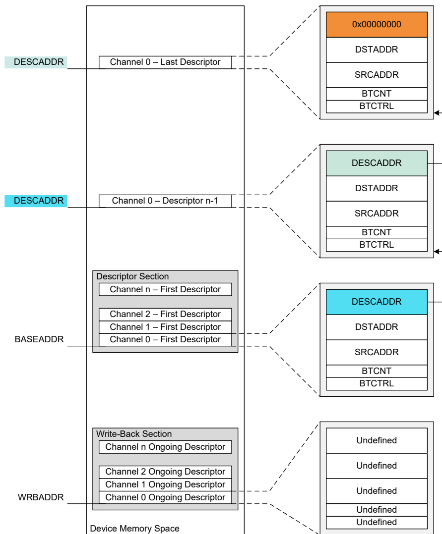
Figure 27-3. Memory Sections
