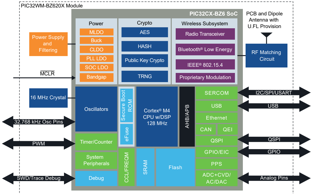
Figure 5-1. PIC32WM-BZ6 Module Block Diagram
