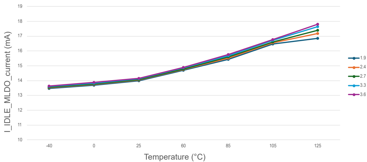
Figure 49-6. Idle Mode Current Consumption in MLDO Mode at FRC 8 MHz
