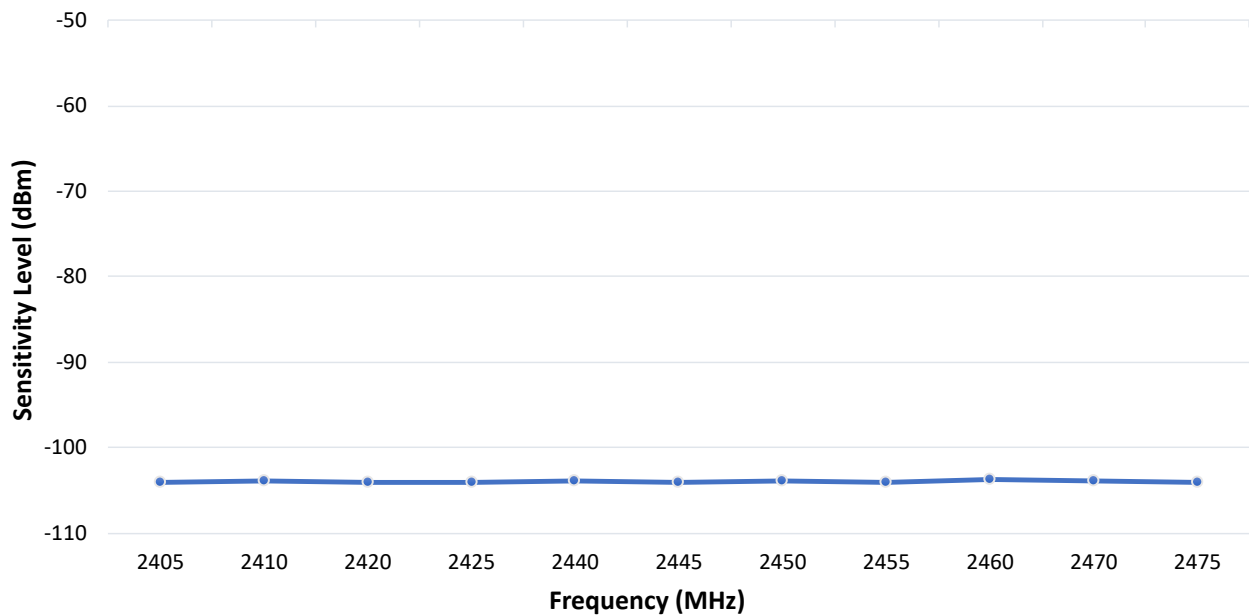
Figure 49-59. Module Zigbee Receive Sensitivity vs. Frequency
