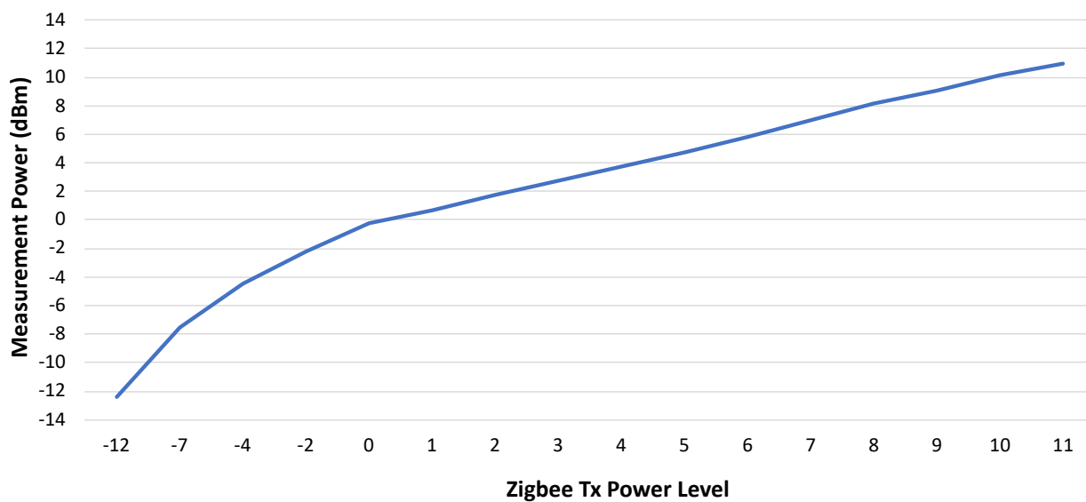
Figure 49-50. Zigbee Transmit Power vs. Power Level
