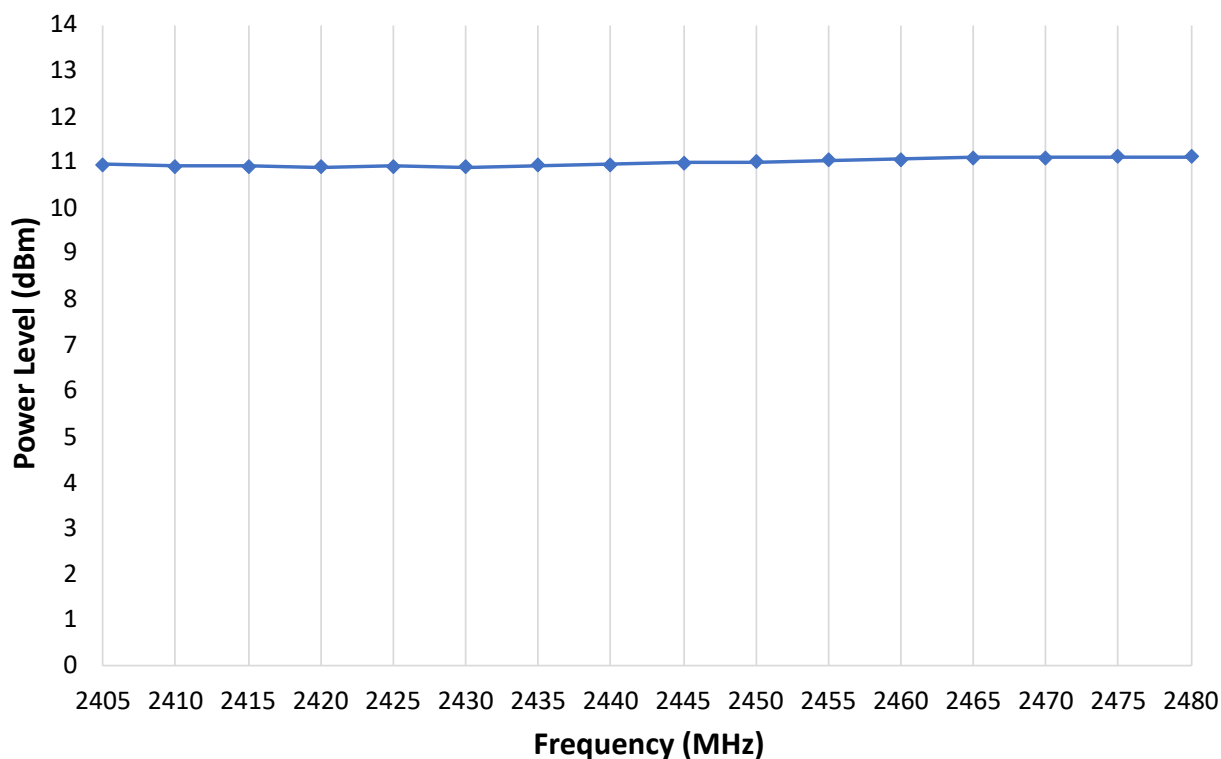
Figure 49-49. Zigbee Transmit Power vs. Frequency
