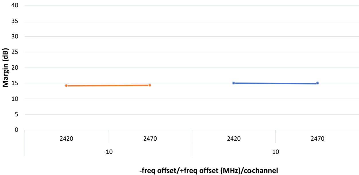
Figure 49-57. Zigbee ACR RX CI 10M Margin
