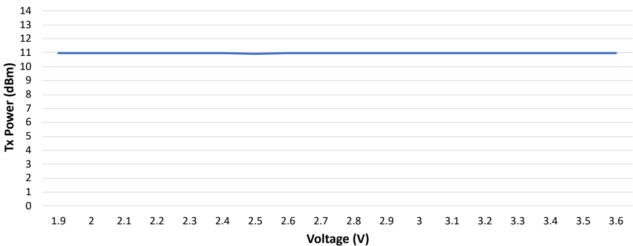
Figure 49-48. Zigbee Transmit Power vs. VDD Supply Voltage
