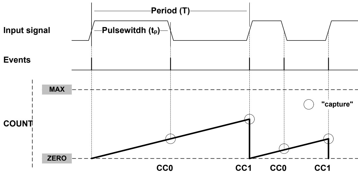
Figure 41-13. PWP Capture
