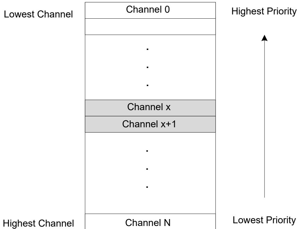
Figure 31-3. Static Priority
