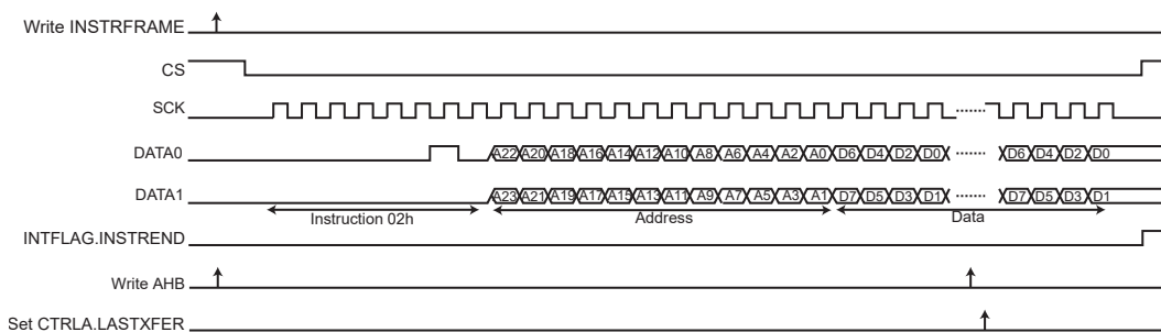
Figure 36-16. Instruction Transmission Waveform 5
