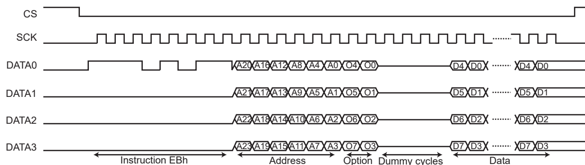
Figure 36-9. Instruction Frame
