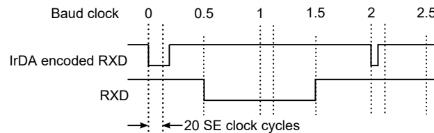
Figure 33-11. IrDA Receive Decoding
