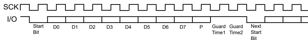
Figure 33-18. T = 0 Protocol without Parity Error
