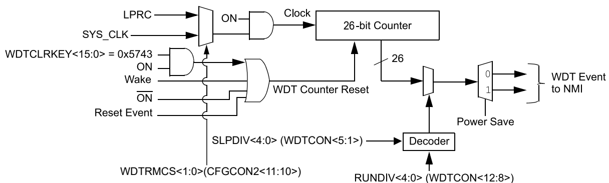
Figure 20-1. Block Diagram
