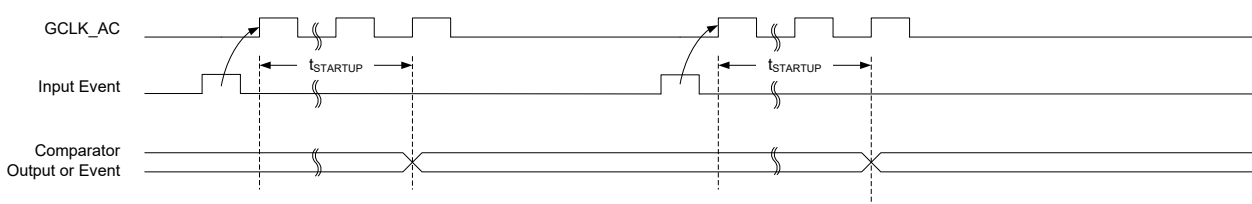
Figure 39-10. Single-Shot SleepWalking
