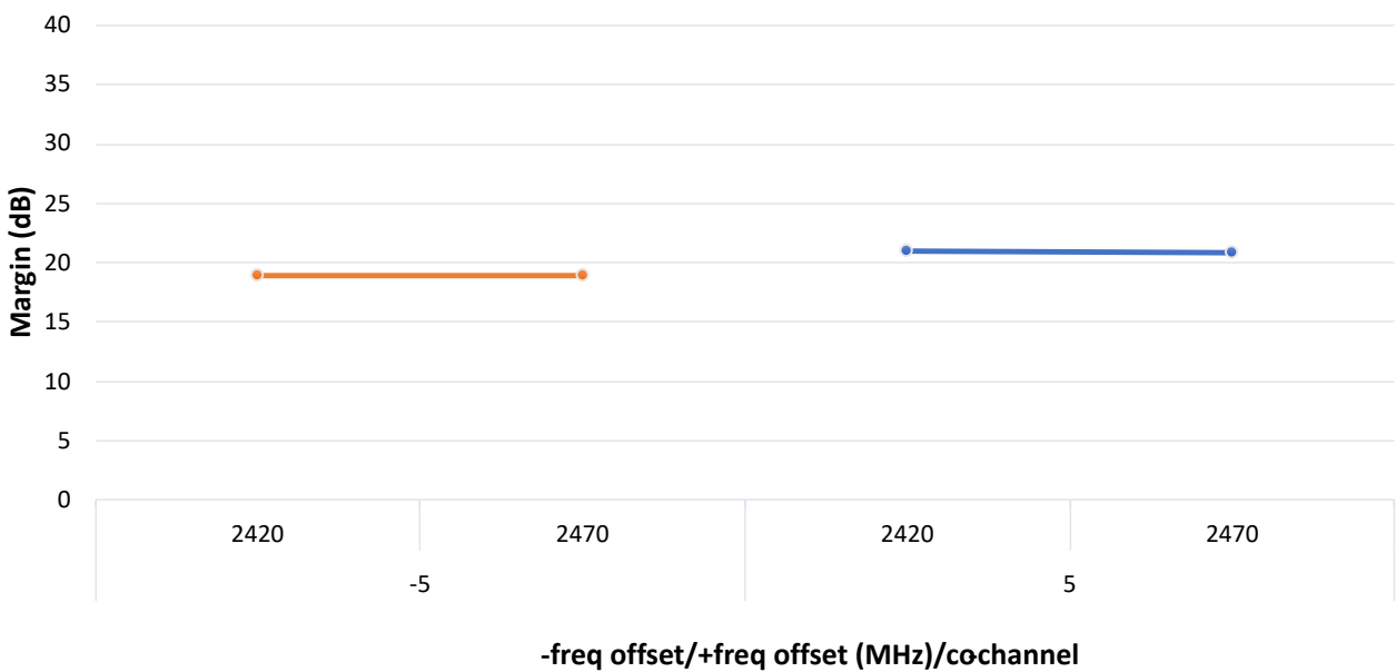
Figure 49-56. Zigbee ACR 5M Margin
