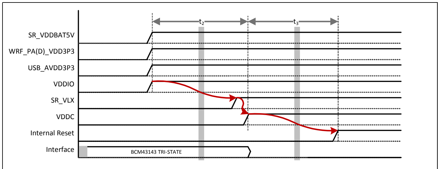
Figure 1. Power-Up Sequence Timing—3V Supply
