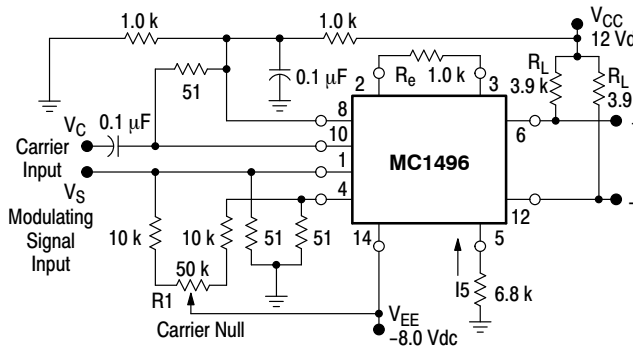
Figure 26. Balanced Modulator-Demodulator
