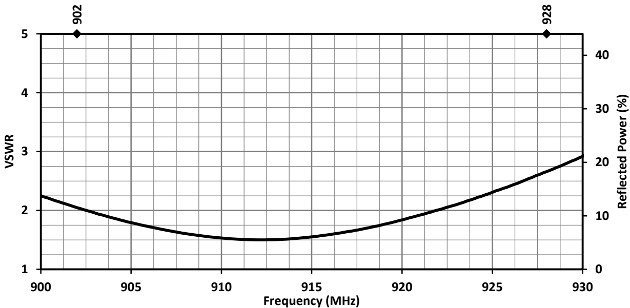
Figure 1. ANT-915-uSP410 VSWR
