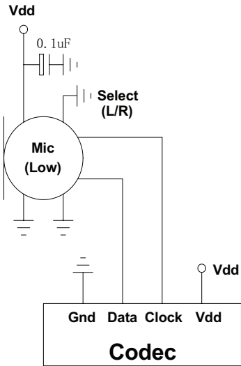
Single Microphone
