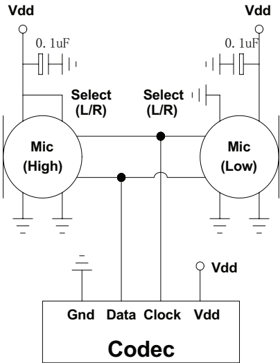
Dual Microphone
