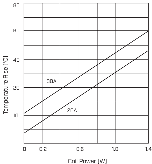
Coil Temperature Rise
