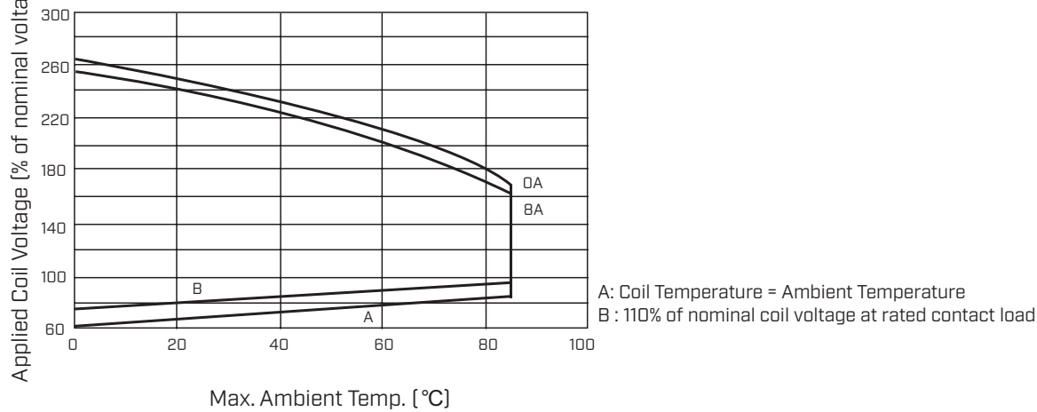
Max Ambient Temp. Vs. Coil Voltage
