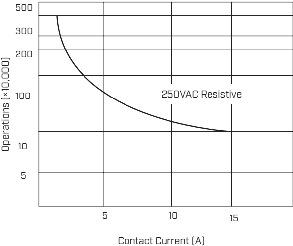
Life Curve
