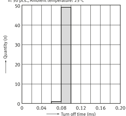
18-4. Turn off time distribution
