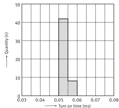
17-5. Turn on time distribution
