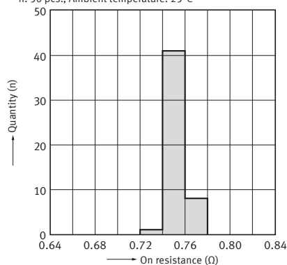
16-5. On resistance distribution
