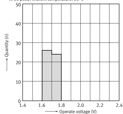
19-4. Operate voltage distribution
