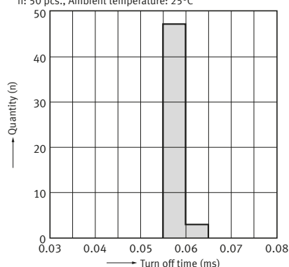
18-5. Turn off time distribution
