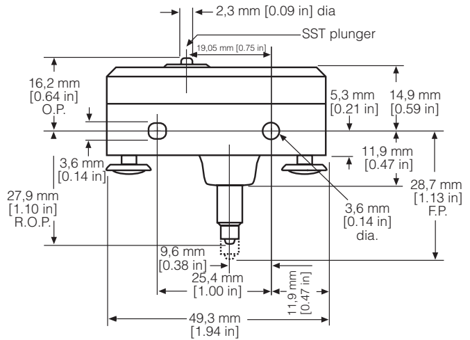
Figure 12. Pin plunger with manual reset
