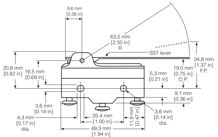
Figure 10. BA/BE Series: Straight lever
