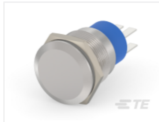
TE Part # 2213763-7 AV19 DPL 3A NO LED
