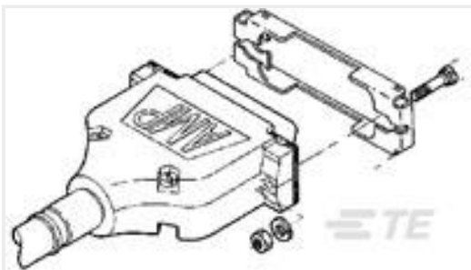
TE Part #1617168-3 JMSCT-18XL = M28776/3-037L
