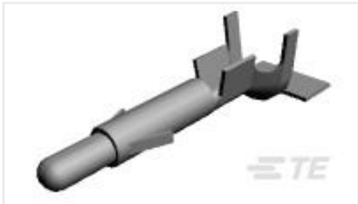
TE Part #350707-7 UMNL SPLIT PIN 20-14 AUBR L/P
