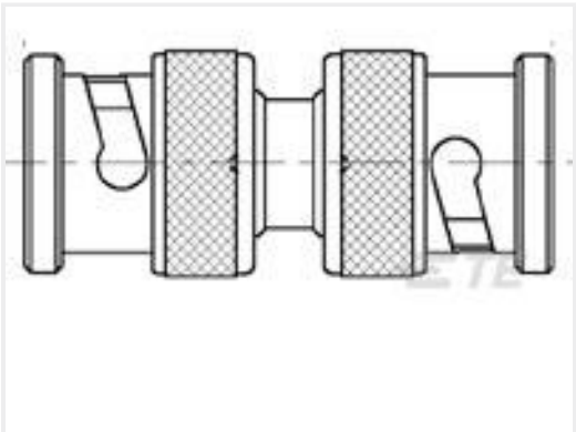
TE Part #1-1478043-0 BNC M TO BNC M ADAPTOR,STR,75 OHM,2G
