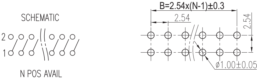
Recommended PCB Layout Top View
