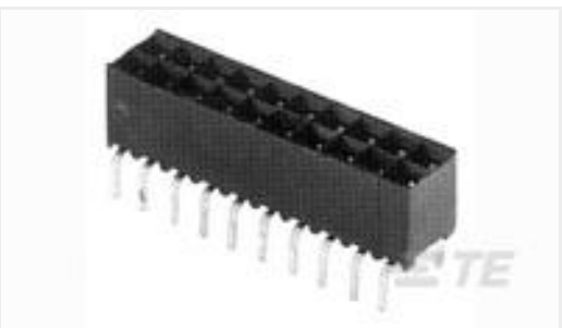
TE Part #1-829264-0 2X10P HV100 REC.CON.B/TE,6.2MM, NO KINK
