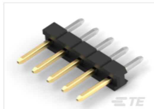
TE Part #2355045-6 6P,2MM,BRK HDR,SRVT,2.8,0.1AU,TB
