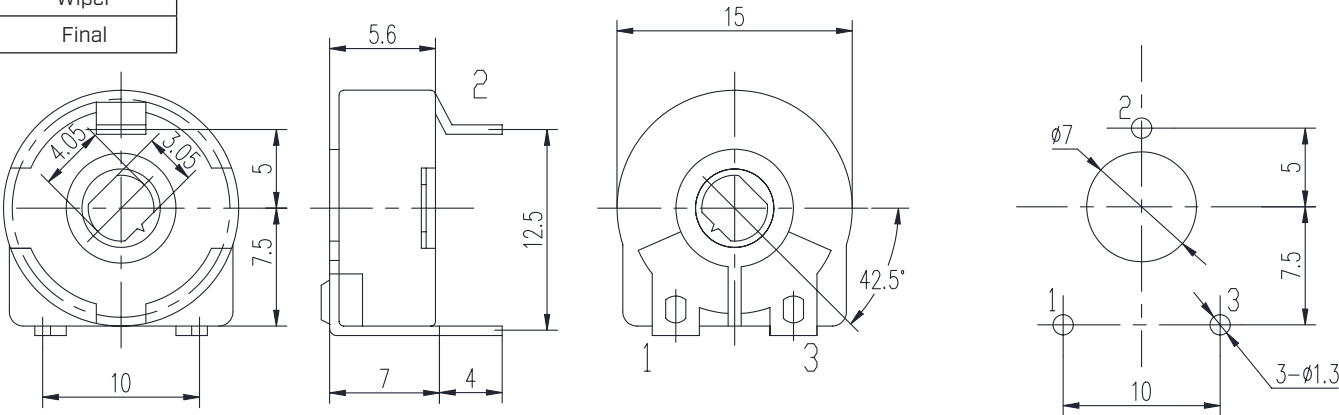
Recommended PCB Layout Top View
