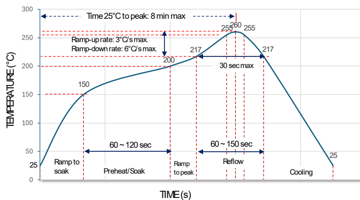
Reflow Profiles
