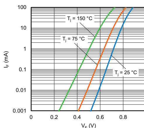
Fig. 6 - Typical Forward Current I_F vs. Forward Voltage V_F
