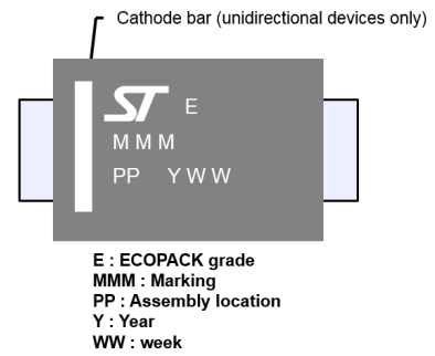
Figure 15. Marking layout
