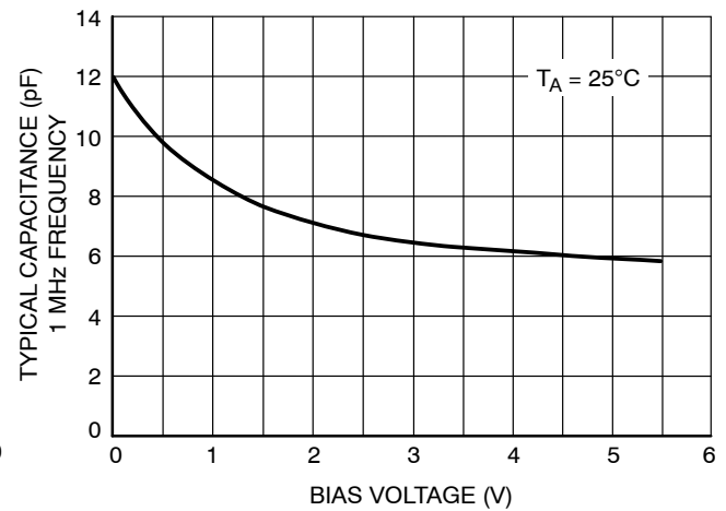
Figure 9. Capacitance
