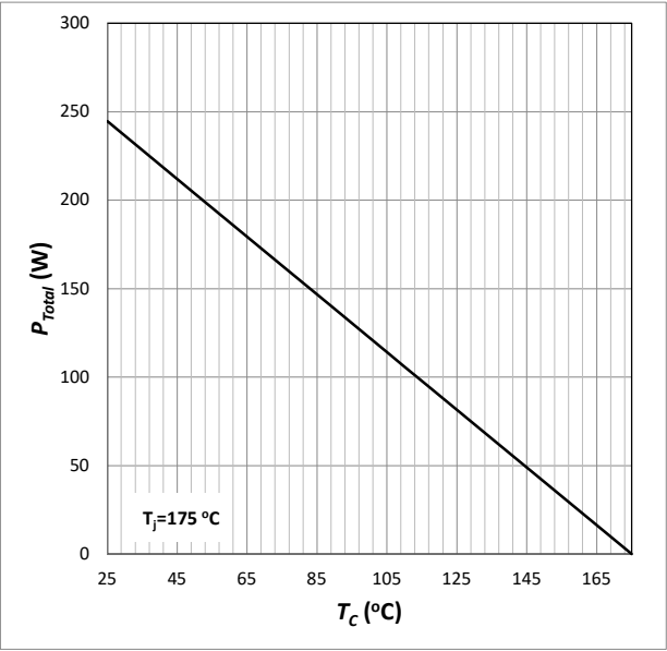
Fig. 4 Power Derating
