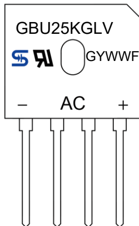
MARKING DIAGRAM
