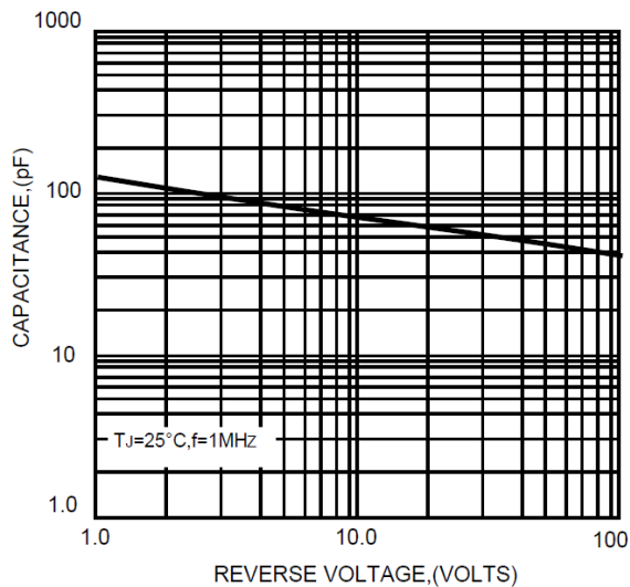
FIG.3-TYPICAL JUNCTION CAPACITANCE
