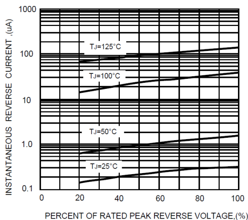
FIG.5-TYPICAL REVERSE CHARACTERISTICS
