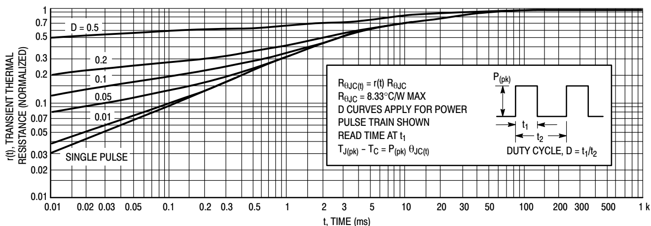
Figure 5. Thermal Response
