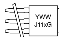
DPAK-3
