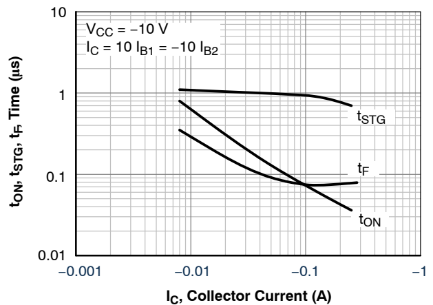
Figure 6. Switching Time
