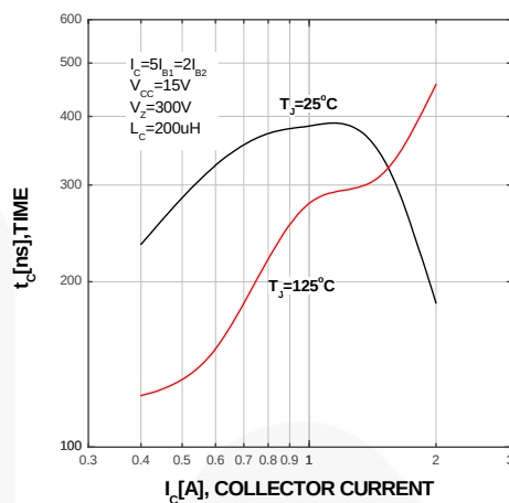
Figure 14. Inductive Switching Time, t_c
