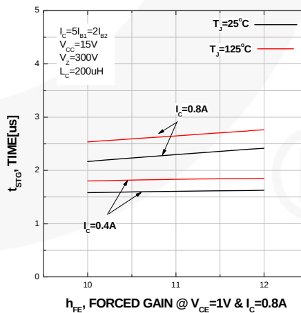
Figure 18. Inductive Switching Time, t_{STG}
