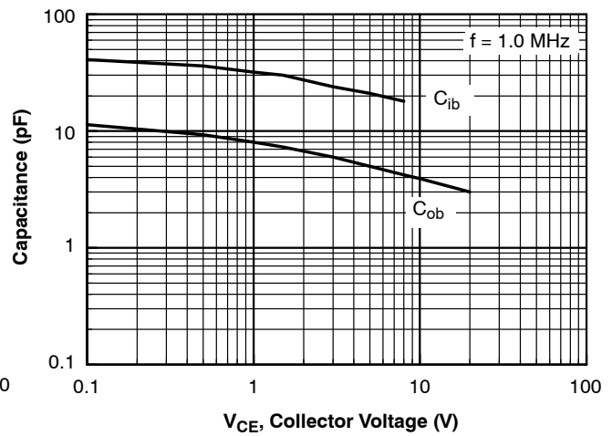
Figure 8. Input and Output Capacitance vs. Reverse Voltage
