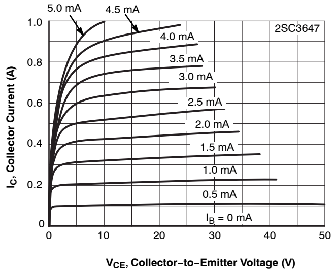
Figure 5. I_C - V_{CE}
