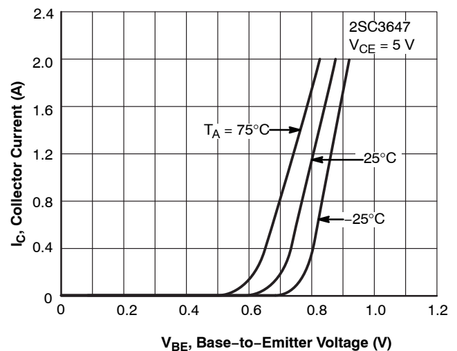
Figure 7. I_C - V_{BE}
