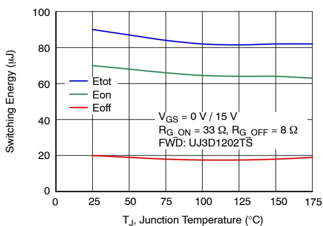
Figure 20. Clamped Inductive Switching Energy vs. Junction Temperature at V_{\text{DS}} = 800 \text{ V} , and I_D = 5 \text{ A}
