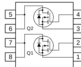
N-Channel MOSFET
