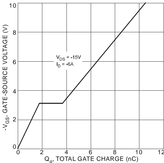
Figure 23. Gate-Charge Characteristics
