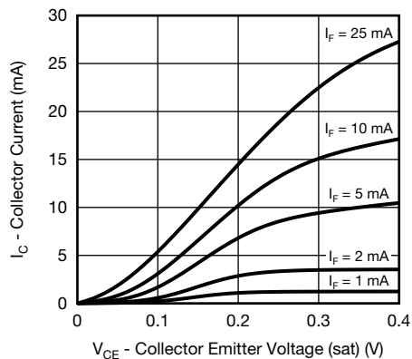
Fig. 6 - Collector Current vs. Collector Emitter Voltage (saturated)
