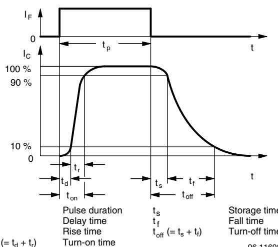
Fig. 3 - Switching Times
