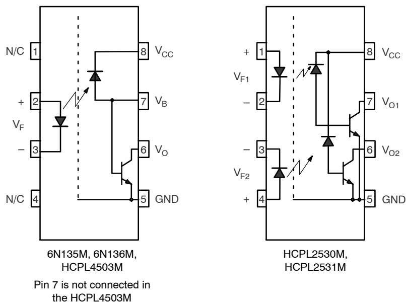
Figure 1. Schematics
