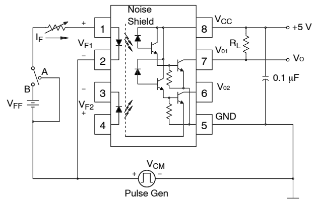
Test Circuit for HCPL-0731
