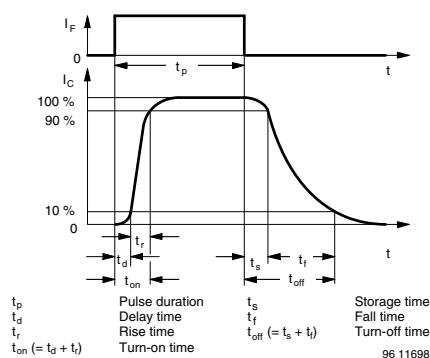
Fig. 2 - Switching Times
