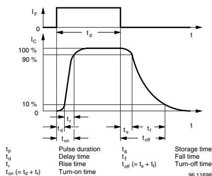
Fig. 2 - Switching Times
