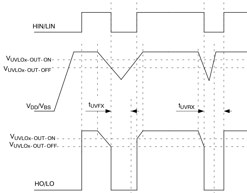
Figure 5. UVLO
