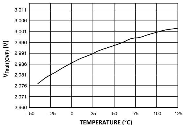
Figure 25. V Fault(OVP) vs. Junction Temperature
