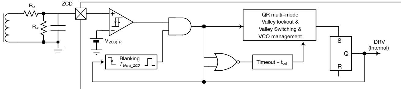
Figure 35. Valley Lockout Detection Circuitry Internal Schematic
