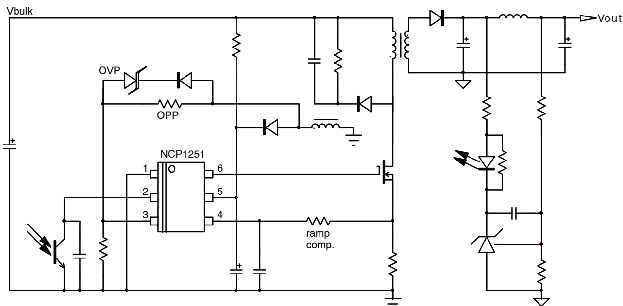
Figure 1. Typical Application Example
