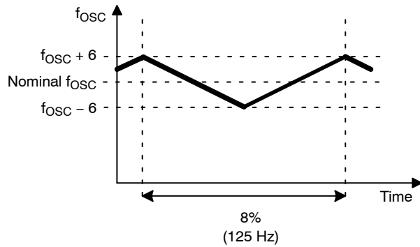
Figure 30. Frequency Jittering
