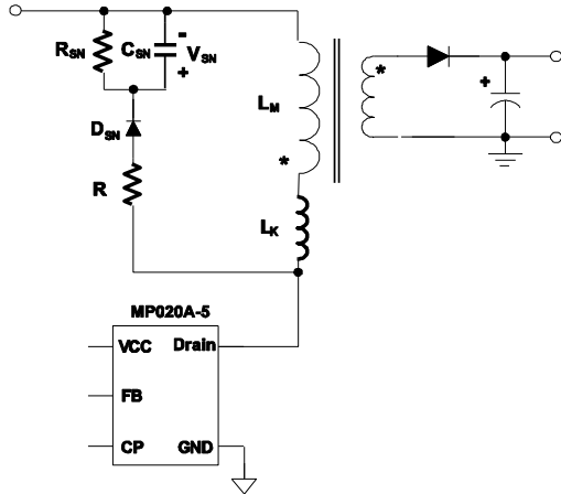
Figure 8: RCD Snubber
